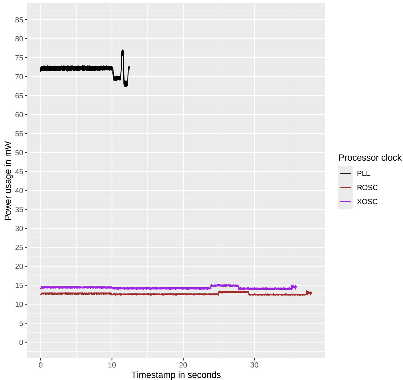
Pico 2 power usage trace running benchmarks according to processor clock
