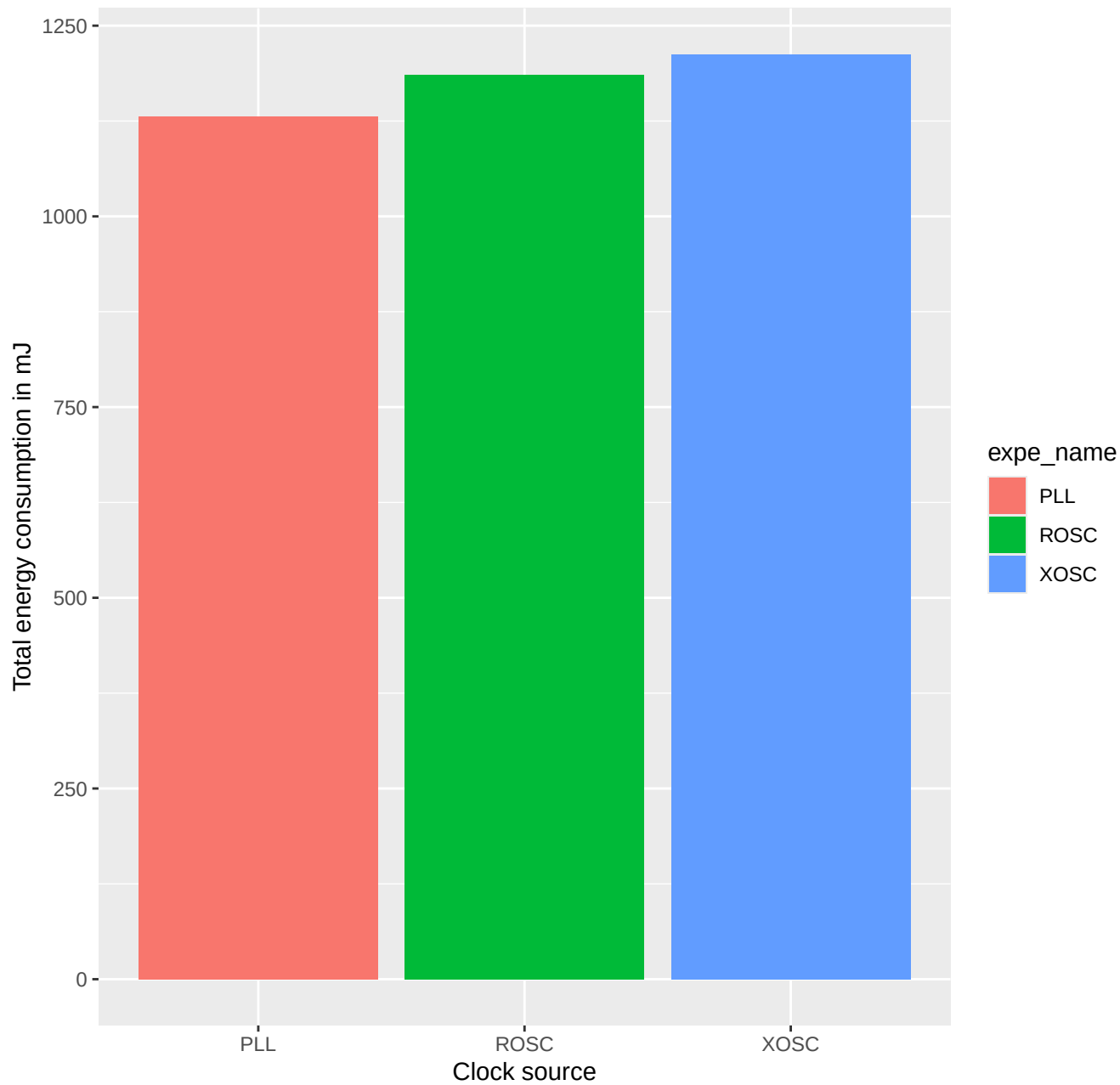
Energy consumption per clock source
