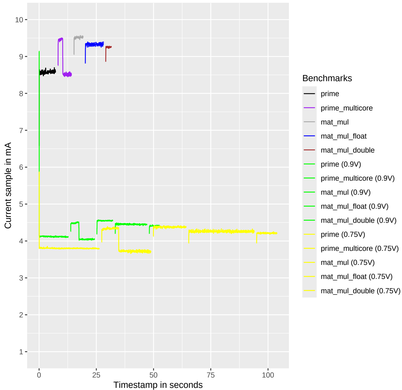
Rosc benchmarks, divider: 1
