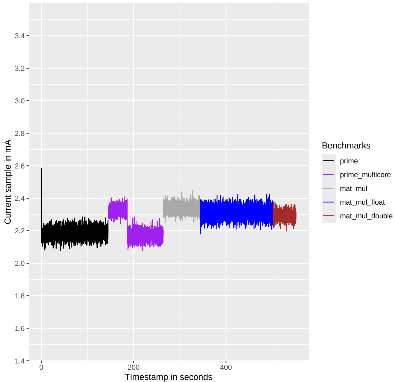
Rosc benchmarks, divider: 20
