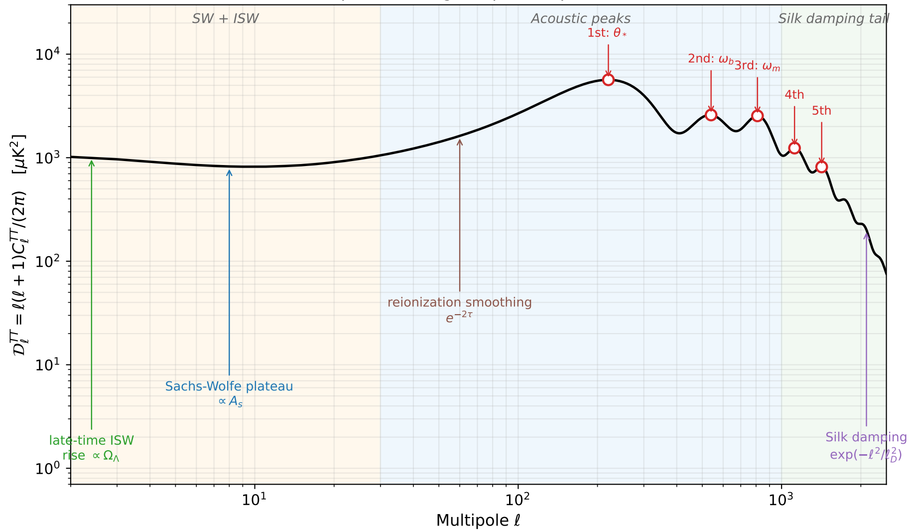
The CMB temperature angular power spectrum, annotated
