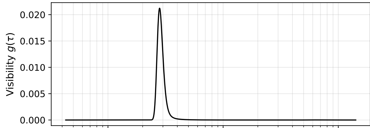
Visibility function and Thomson opacity
