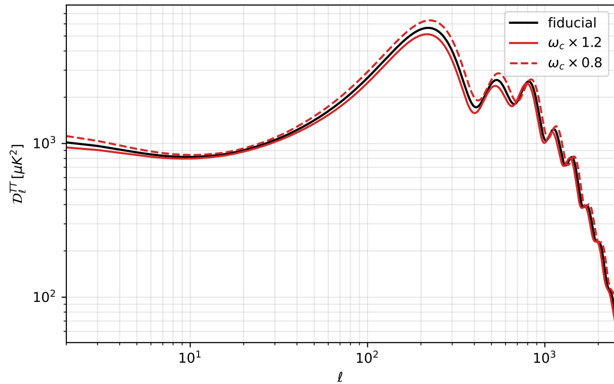
TT dependence on \omega_c
