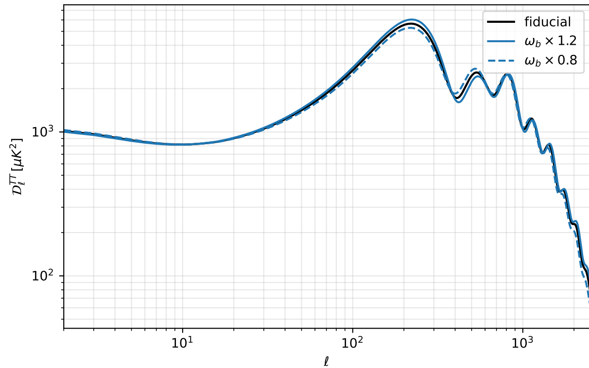
TT dependence on \omega_b
