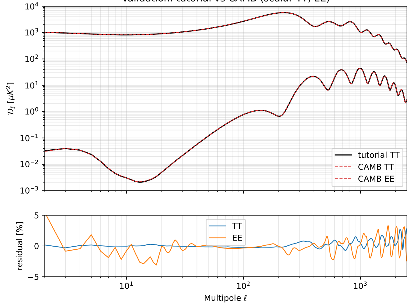
Validation: tutorial vs CAMB (scalar TT, EE)
