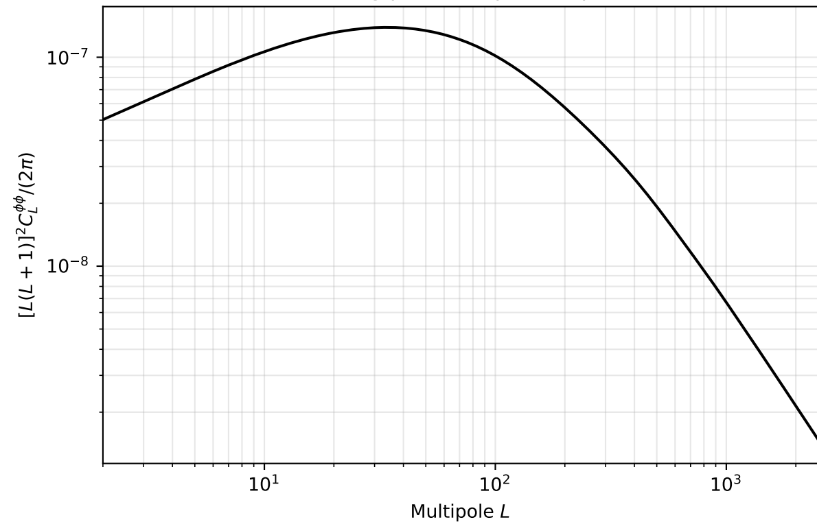
CMB lensing potential power spectrum
