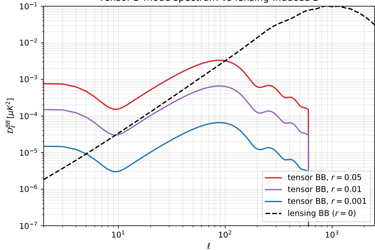
Tensor B -mode spectrum vs lensing-induced B
