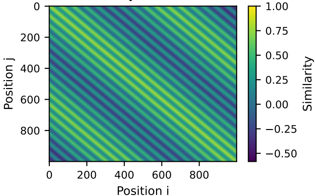
Cosine Similarity Between Positions
