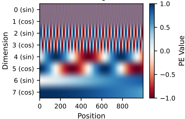
Positional Encoding Matrix (8D)
