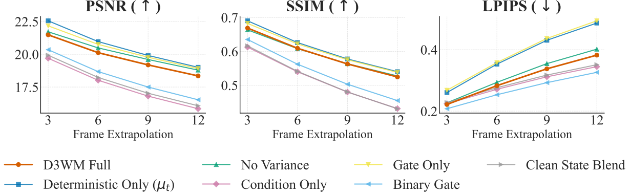
Figure 6: Ablations of D3WM method. The D3WM Full provides the best balance of structural similarity, signal fidelity and perceptual realism.
