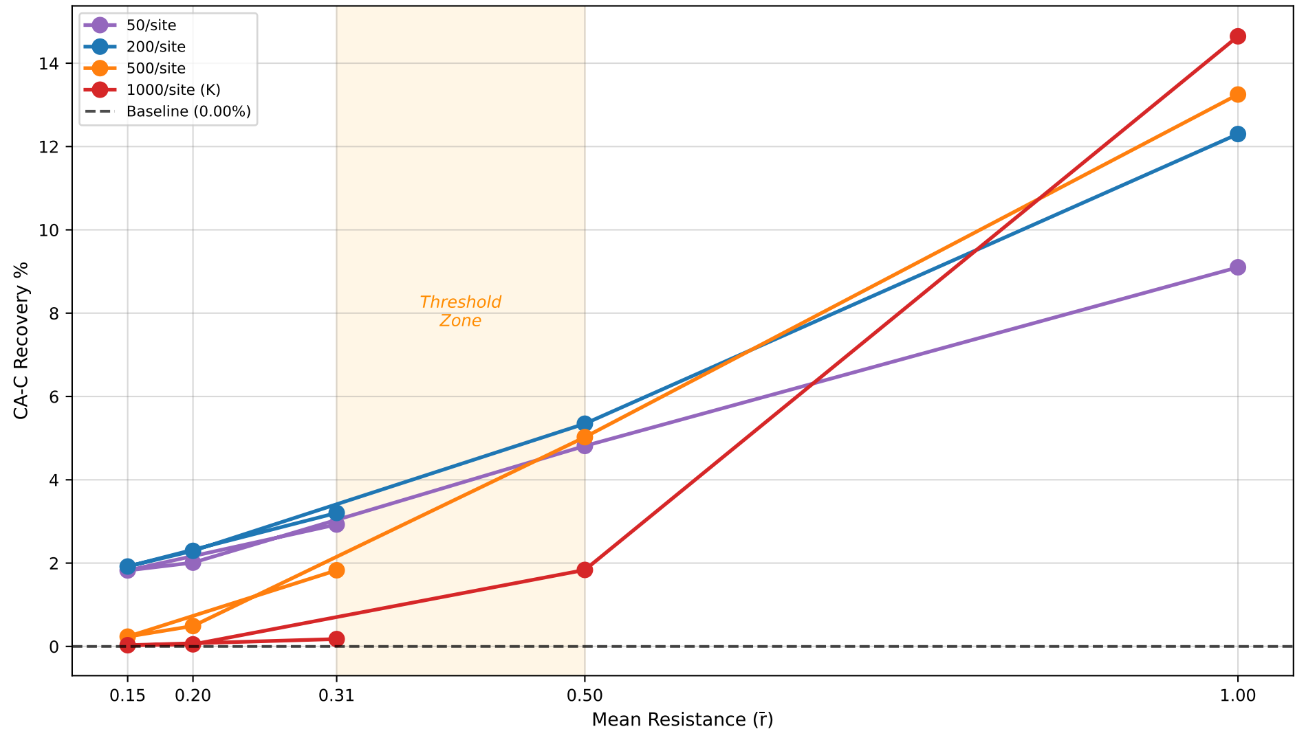
Resistance Threshold for CA-C Recovery (L1)
