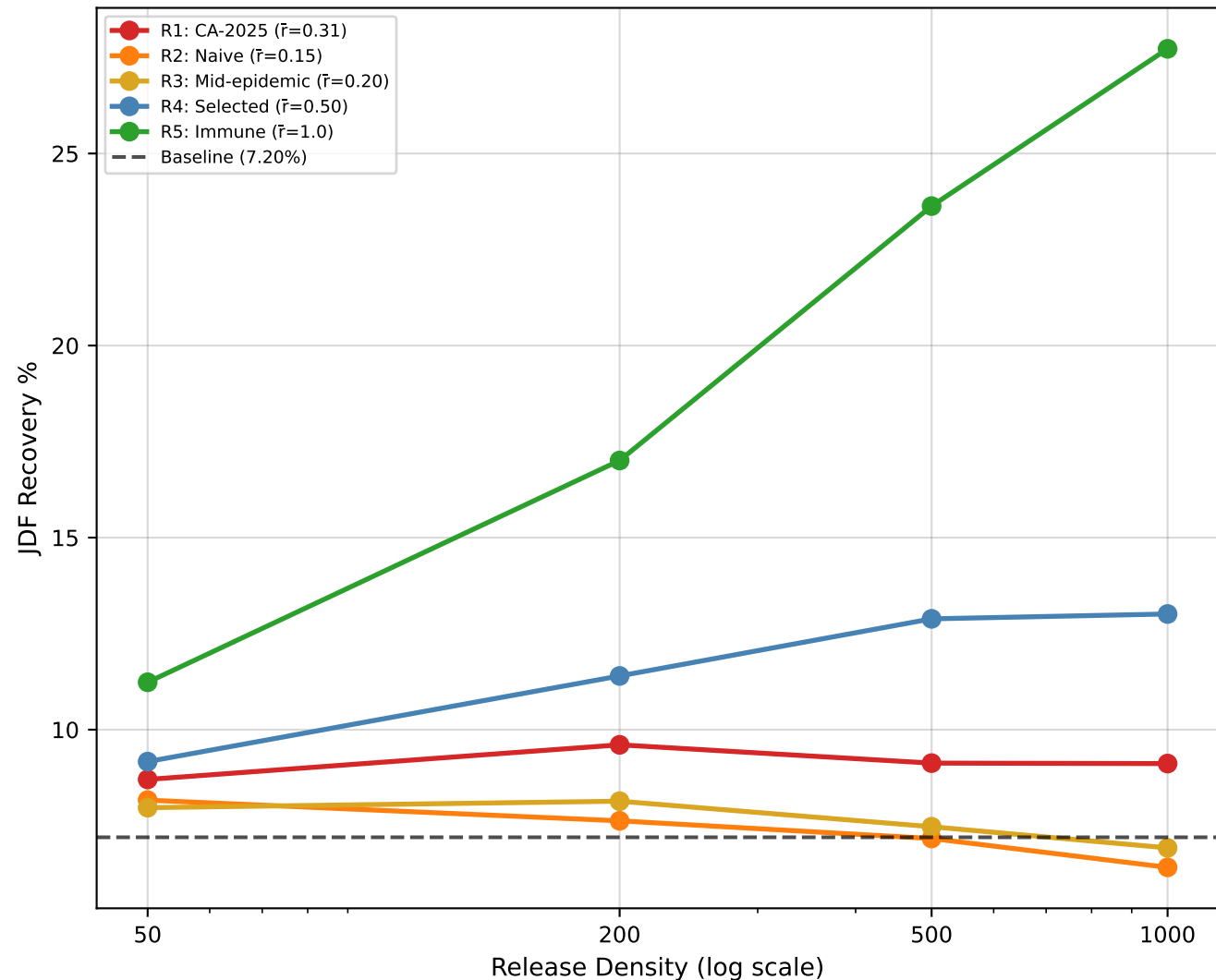
(b) L2: JDF Recovery
