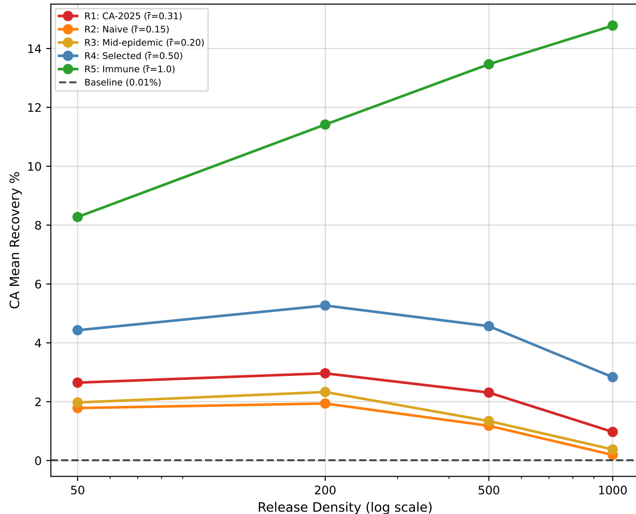
(a) L1: California Mean Recovery
