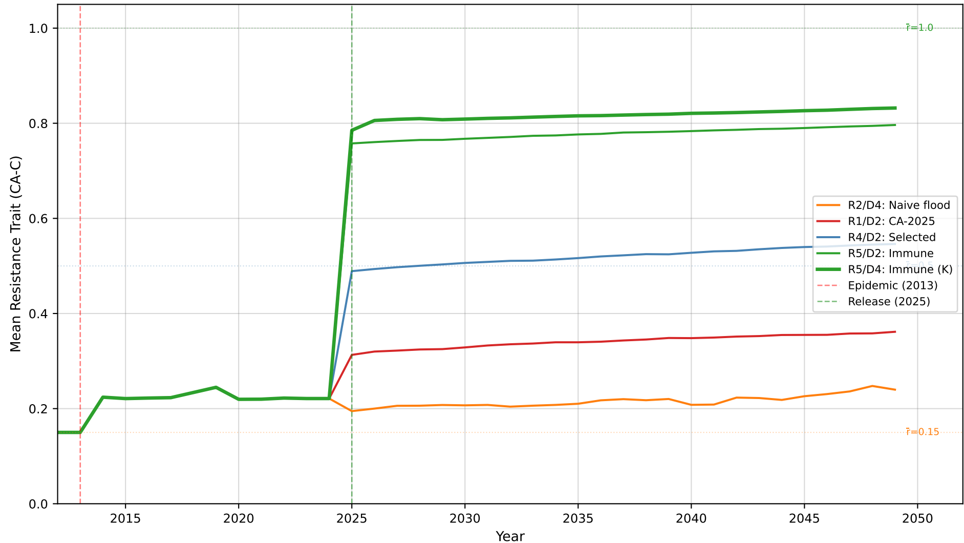
Genetic Evolution of Resistance at CA-C After Release
