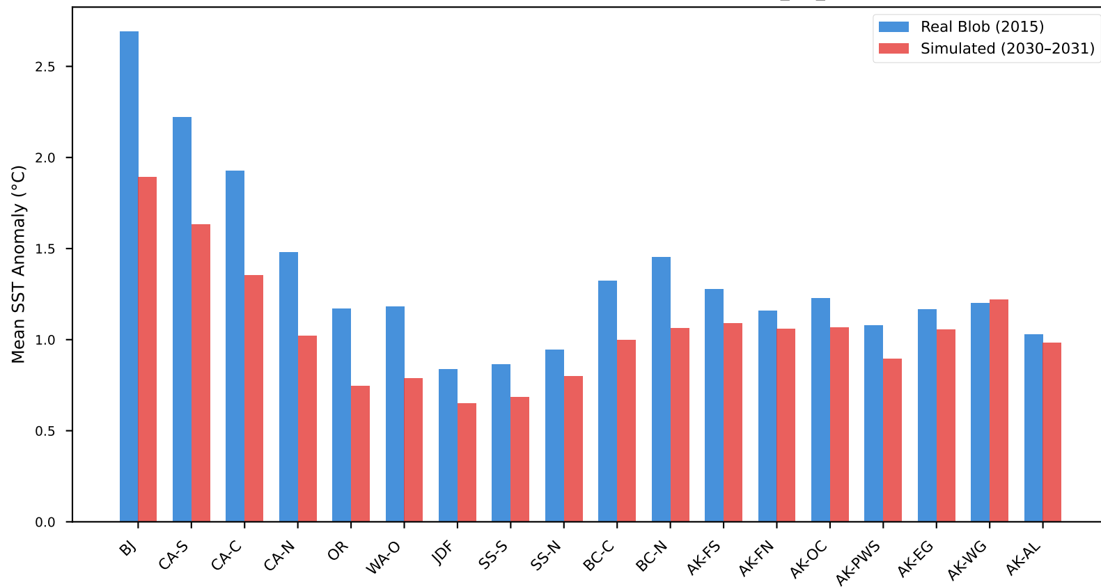
Peak Anomaly: Real Blob vs. Simulated MHW_S1_MED
