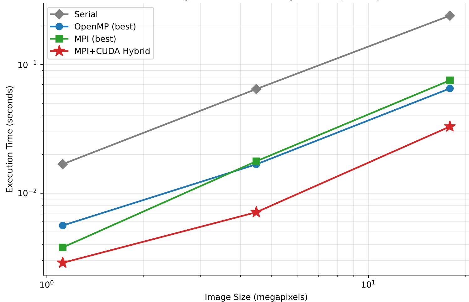
Execution Time vs Image Size (best configuration per implementation)
