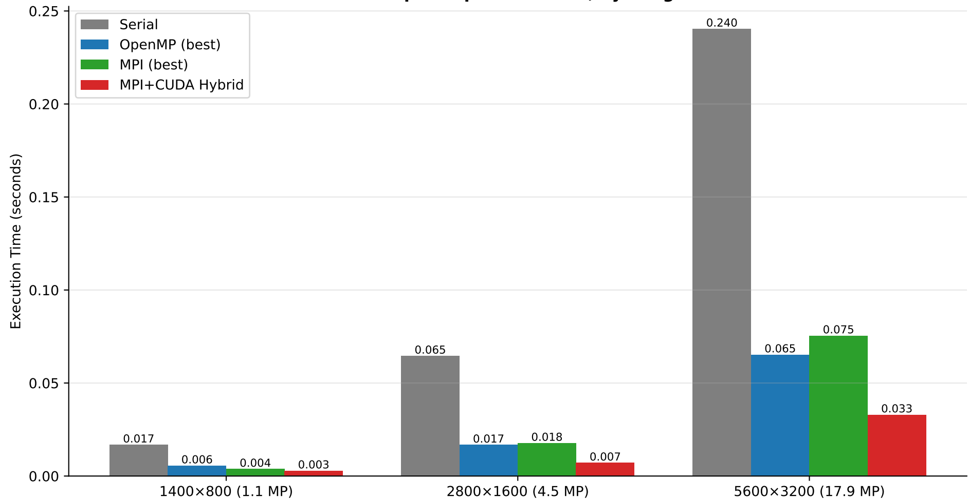
Best Time per Implementation, by Image Size
