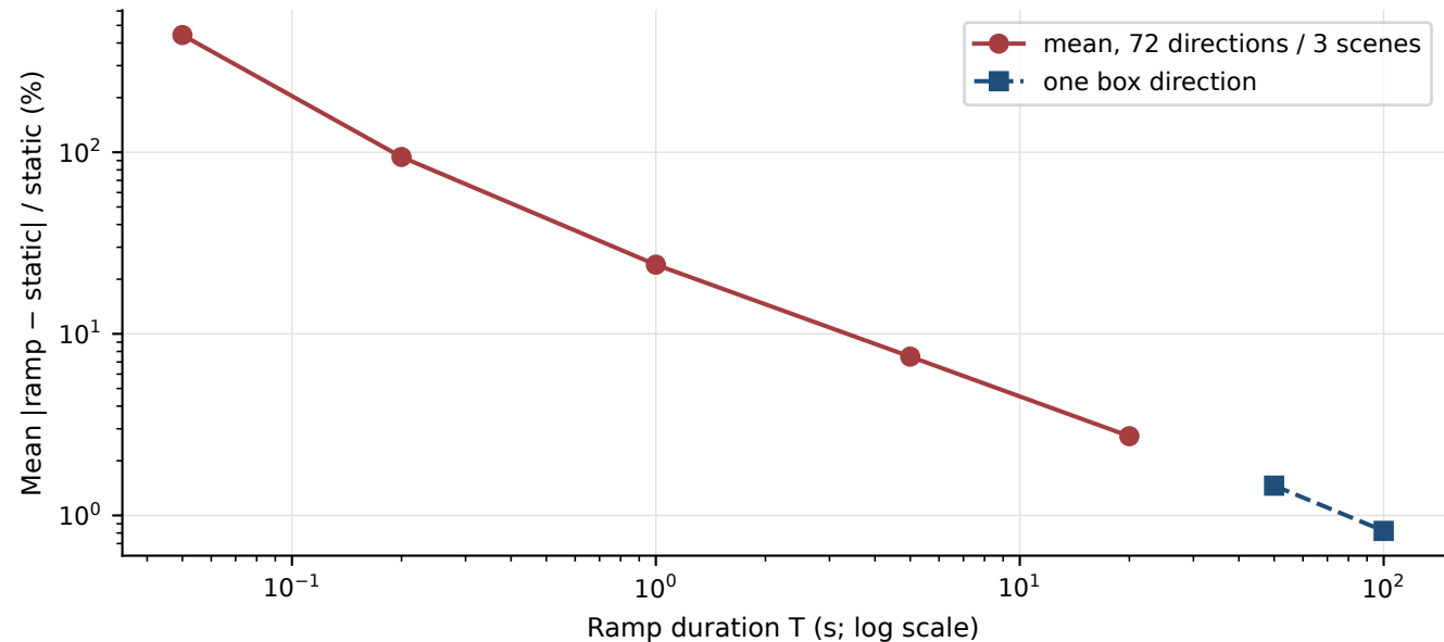
Ramp duration and dynamic excess load
