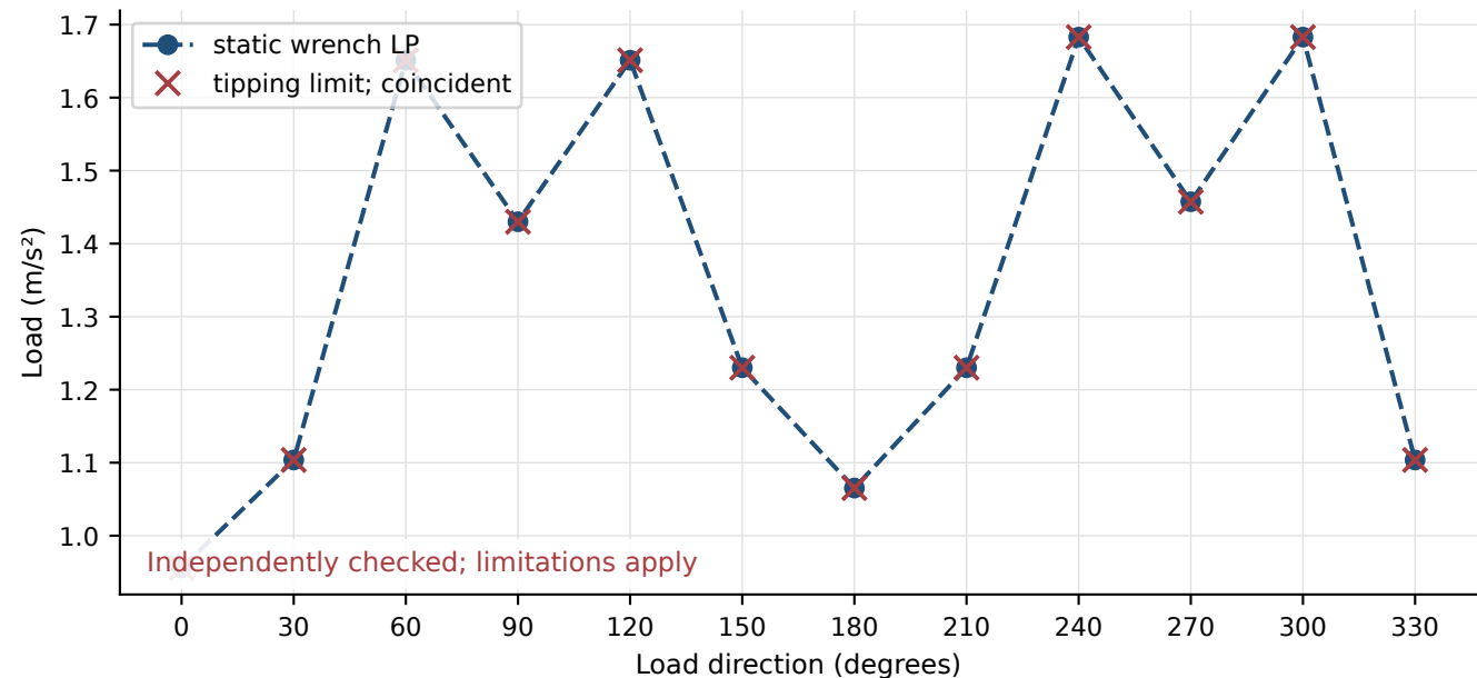
Humanoid double support: static limit by direction
