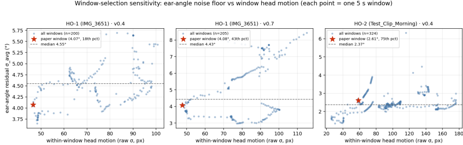
Figure 4: Ear-angle residual \sigma_{\text{avg}} for every 5 s window slid across the target’s detected span, versus within-window head motion. Red star: the hand-picked paper window; dashed line: the median window. Across all windows and both clips \sigma_{\text{avg}} stays a small fraction of the SPFES 40° band and rises only modestly with head motion — the reported noise floor is not an artifact of selecting the stillest segment.
