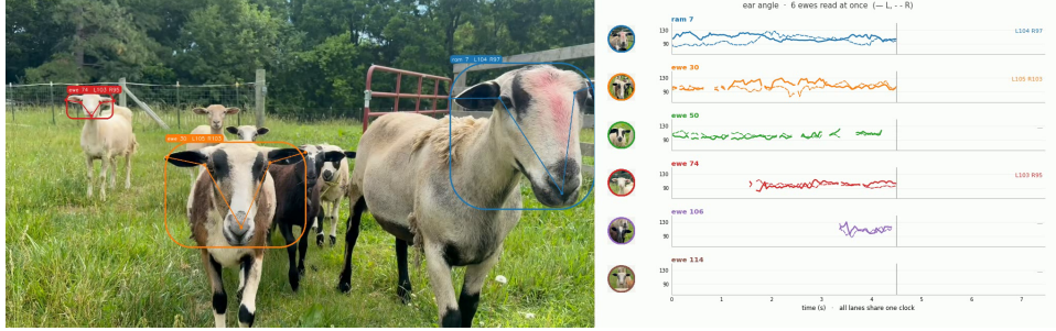
Figure 1: SamSeesSheep pipeline output on held-out clip HO-2 (Table 3): simultaneous ear-angle monitoring of six animals. Left : the supervision-annotated flock with bounding boxes, per-animal labels (including left/right ear angles in degrees), and five-keypoint skeletons (nose, ear bases, ear tips). Right : a six-lane synchronized ear-angle chart with dual traces per lane (solid = left ear, dashed = right ear) and per-animal thumbnails. The frame is a still extracted from the rendered video synced-lanes-6ewes-pro-Test_Clip_Morning.mp4 (2036×640 px, 7.5s; see Data Availability). The figure demonstrates the pipeline’s end-to-end path: ambient pasture video → foundation-model annotation → human review → multi-animal time-series ear-angle extraction, running on an edge GPU with a ~6 MB model.
