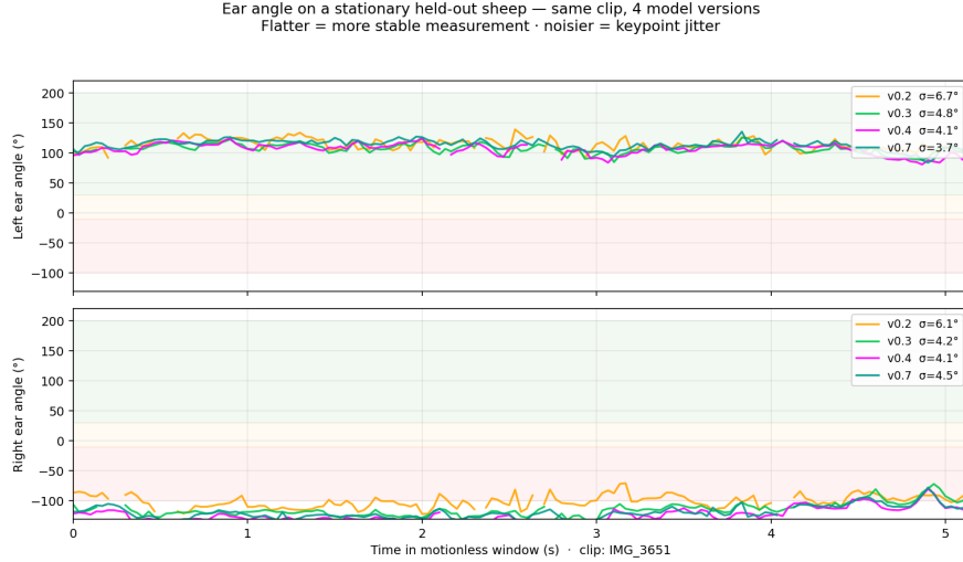
Figure 3: Ear angle over the motionless window on HO-1 for v0.2, v0.3, v0.4, and v0.7. Flatter traces indicate a more stable measurement; noisier traces indicate keypoint jitter. The large v0.2→v0.4 improvement is visible, while v0.7 overlaps v0.4 — consistent with the post-v0.4 plateau (Table 7). Legend \sigma values are residual standard deviations. Shaded bands are the SPFES reference zones (green \geq 30^\circ , amber -10^\circ to 30^\circ , red \leq -10^\circ ); they are literature reference bands, not diagnostic cutoffs.
