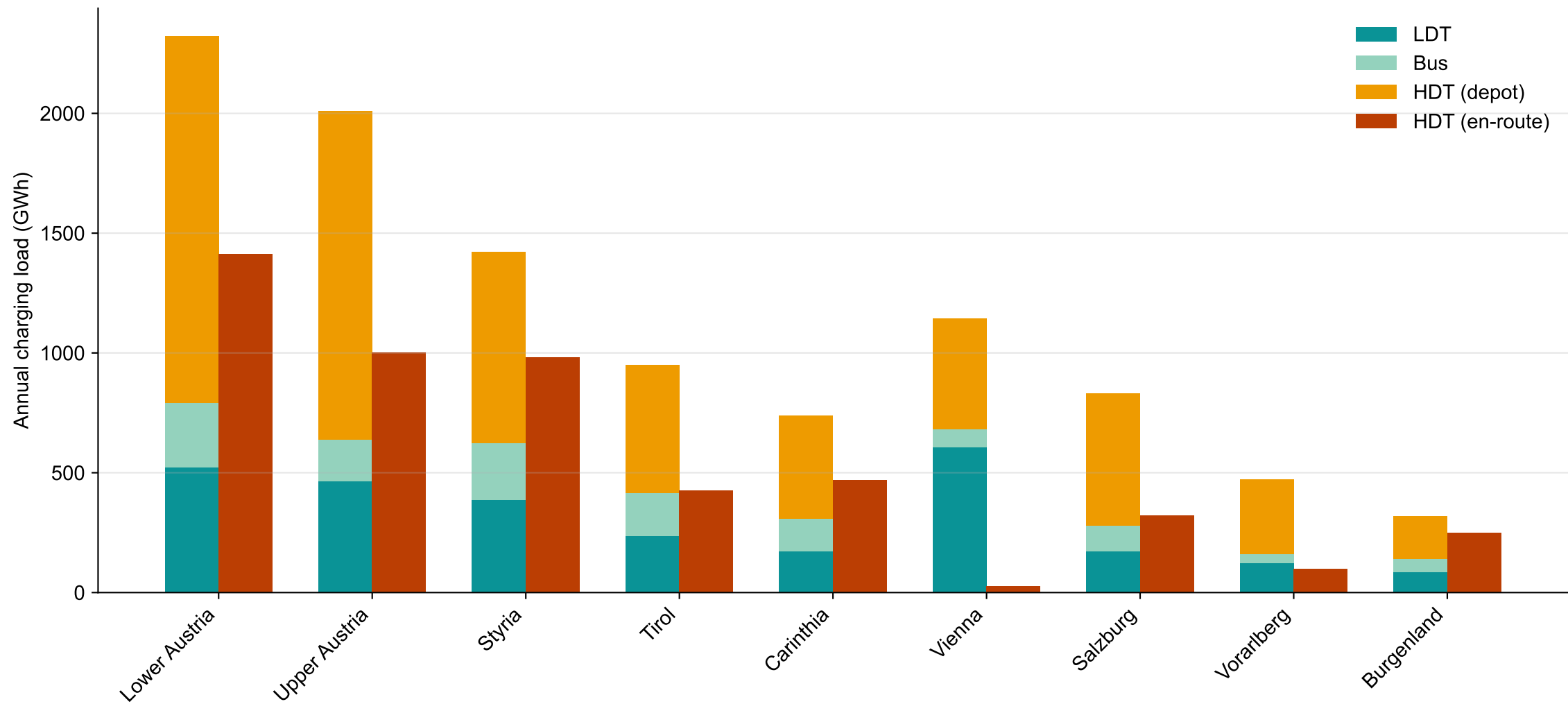
Provincial charging load: depot vs. en-route
