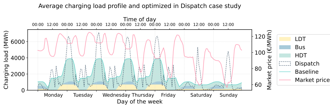
Figure 4.34.: Aggregated weekly charging demand profile of the commercial BEV fleet under baseline assumptions and with market-price-coordinated charging, together with the average day-ahead market price.
