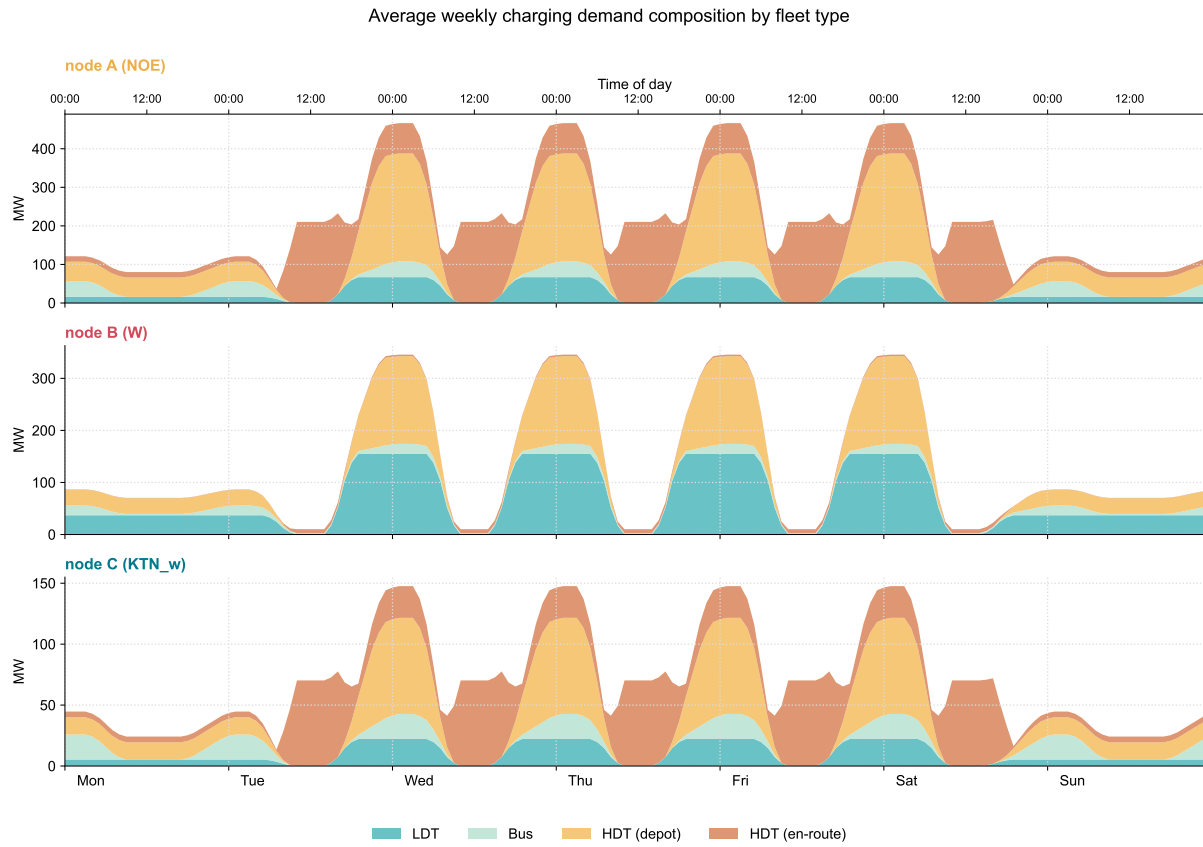
Figure 4.36.: Composition of the weekly charging demand by fleet type (light-duty trucks, heavy-duty trucks, buses) for three selected locations in Austria.
