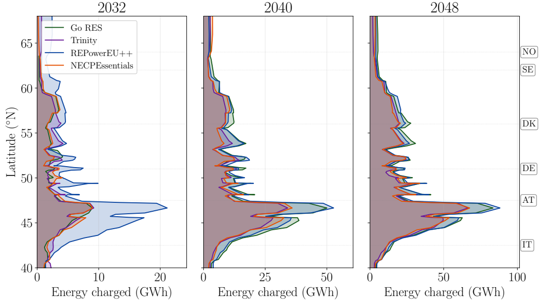
Figure 4.26.: BET energy charged by latitude for the four energy system scenarios across three time horizons (2032, 2040, 2048). Country codes indicate approximate latitude along the Scandinavian-Mediterranean corridor.
