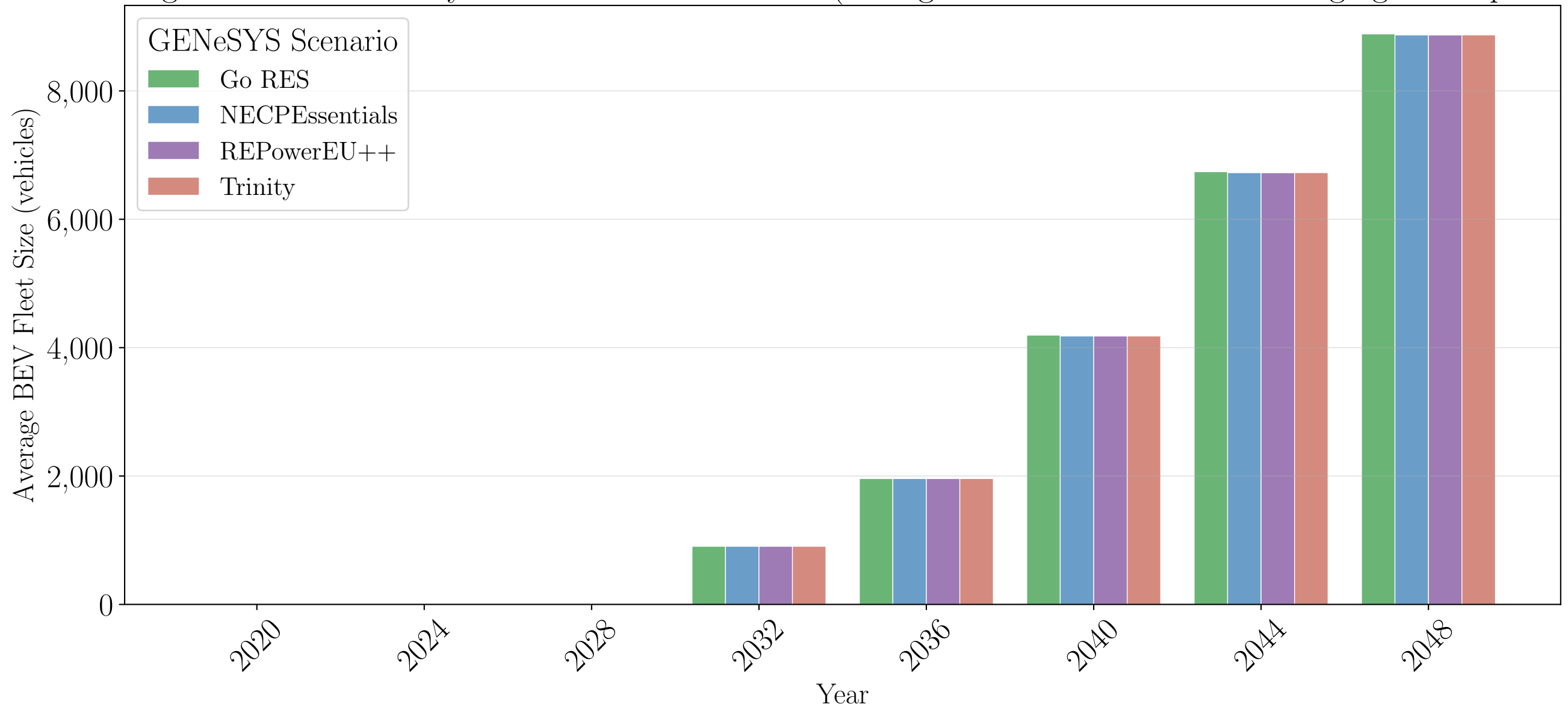
Average BEV Fleet Size by decarbonization scenario (averaged across tech cost and charging markup levels)
