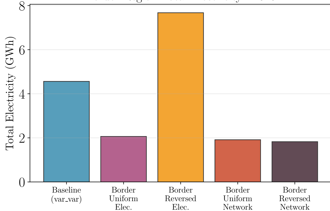
Border Region Total Electricity - 2040
