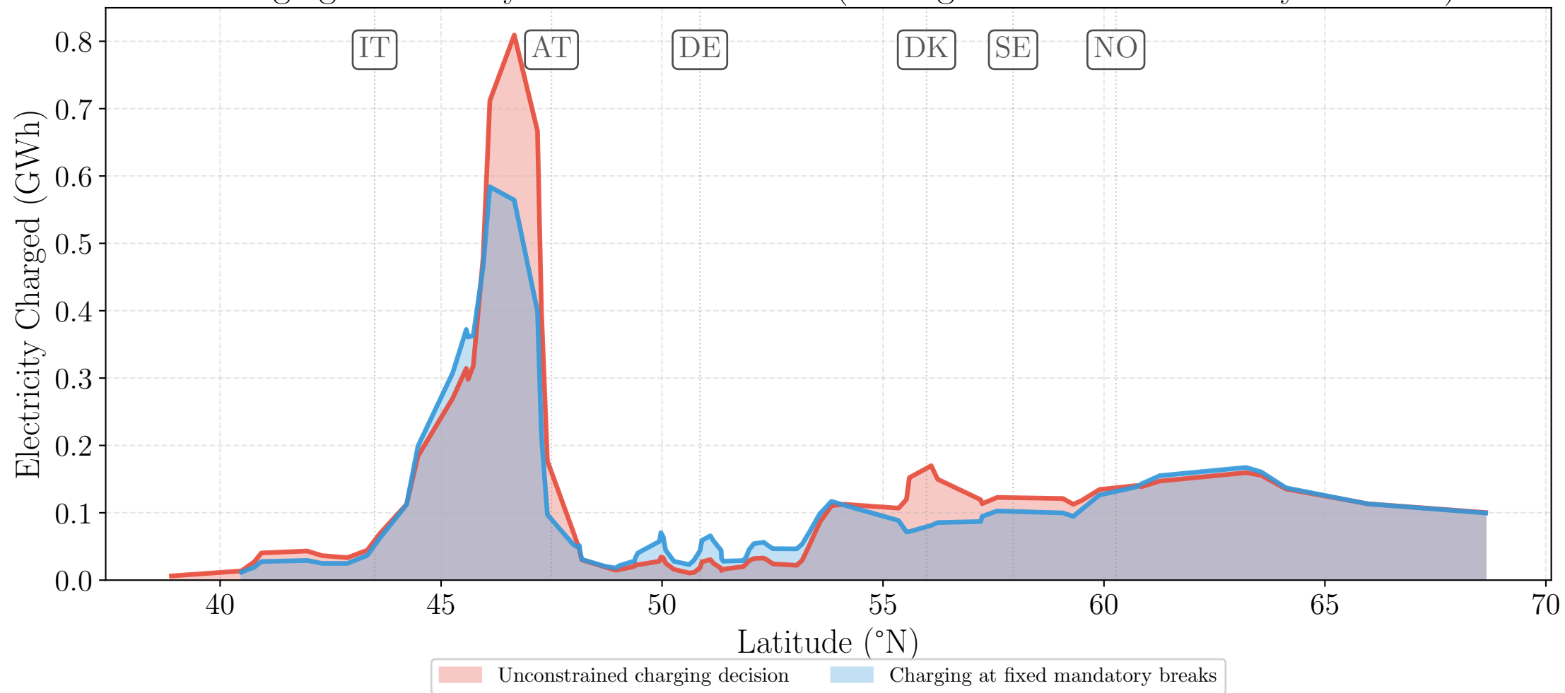
Charging Demand by Latitude: Year 2040(Average across 24 uncertainty scenarios)
