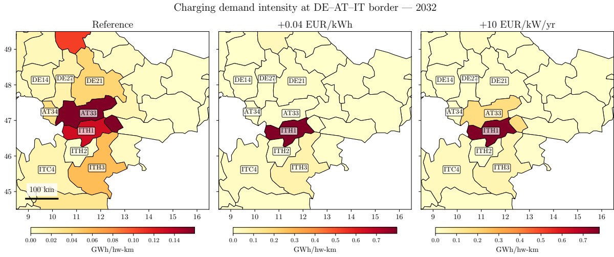
Figure 4.32.: Charging demand intensity (GWh/highway-km) at the DE-AT-IT border region in 2032 (REPowerEU++ scenario). Three panels compare the System-optimal (unconstrained) allocation and the highest electricity price and grid charge premiums. Each panel uses an independent colour scale.
