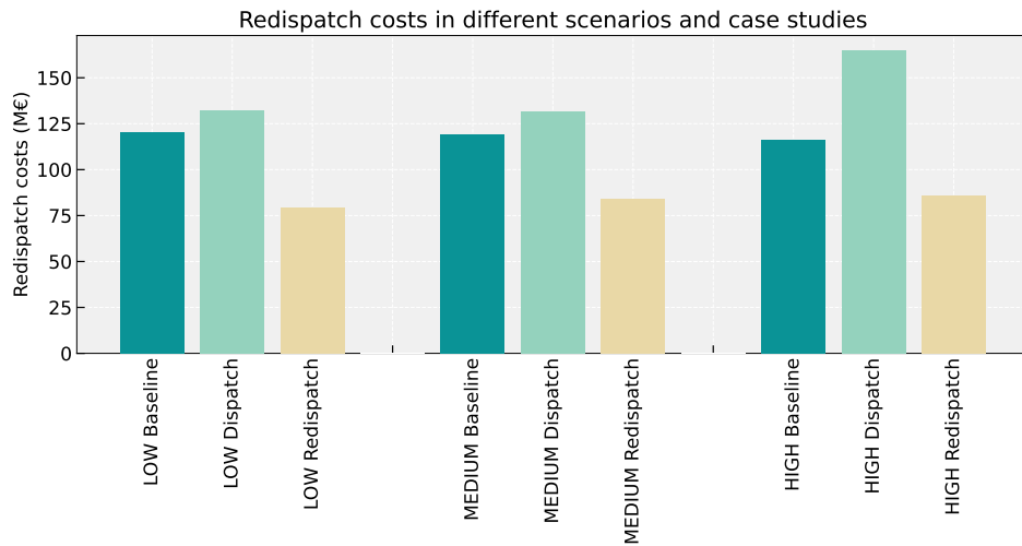
Figure E.6.: Comparison of redispatch costs for different electrification scenarios and case studies for Austria in 2040.
