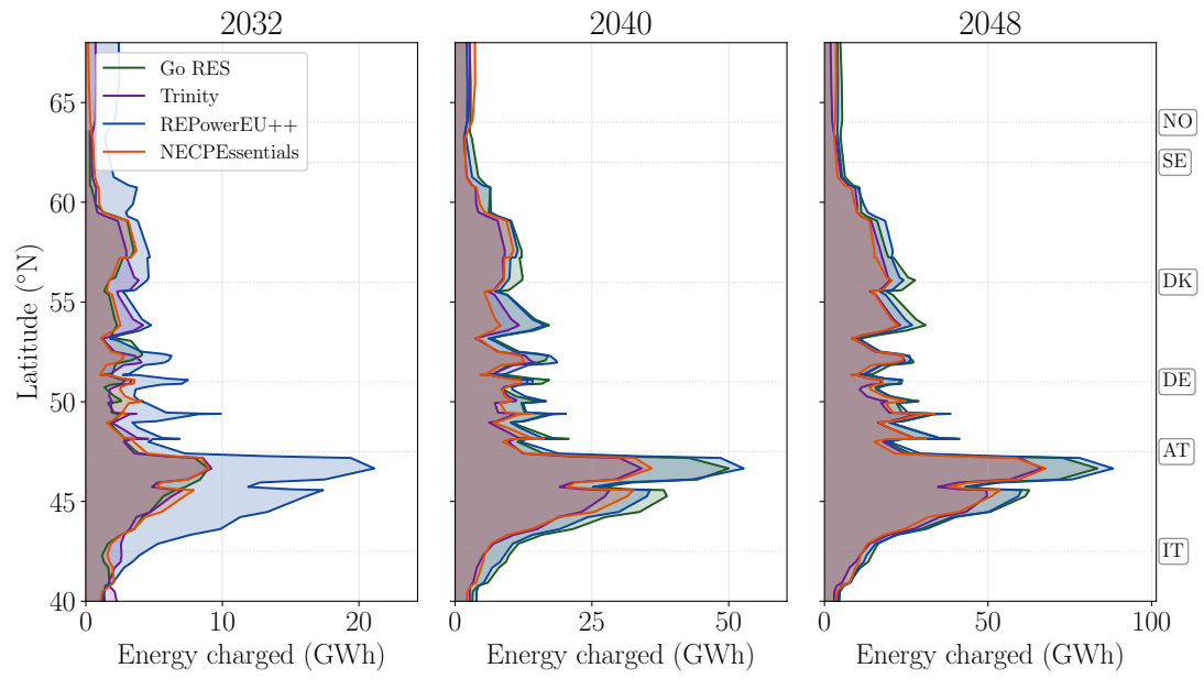
Figure 4.25.: BET energy charged by latitude for the four energy system scenarios across three time horizons (2032, 2040, 2048). Country codes indicate approximate latitude along the Scandinavian-Mediterranean corridor.
