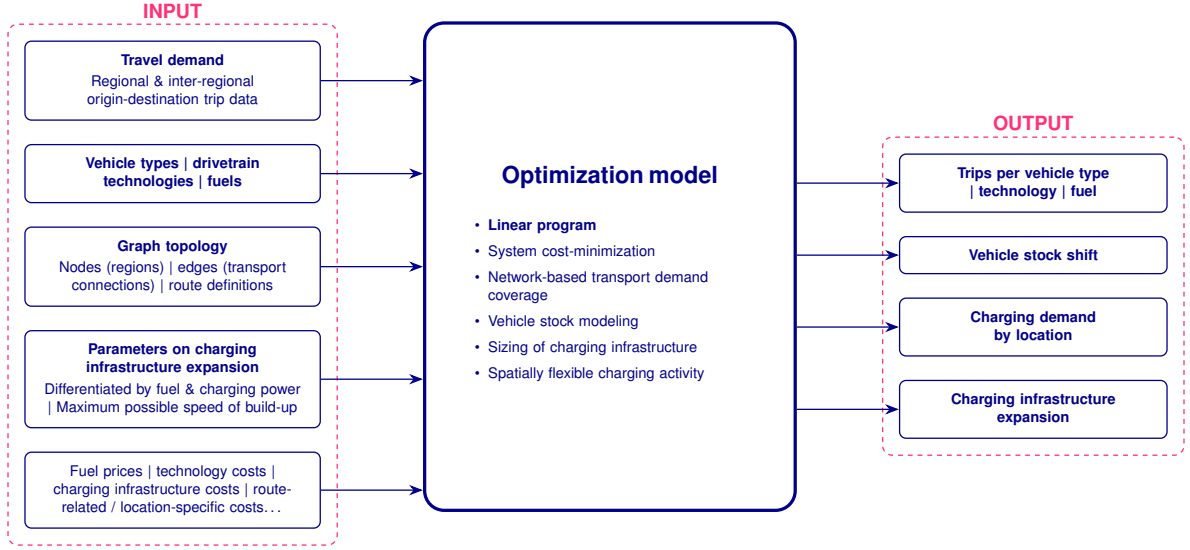
Figure 3.3.: Input-output relations of the core optimization model.
