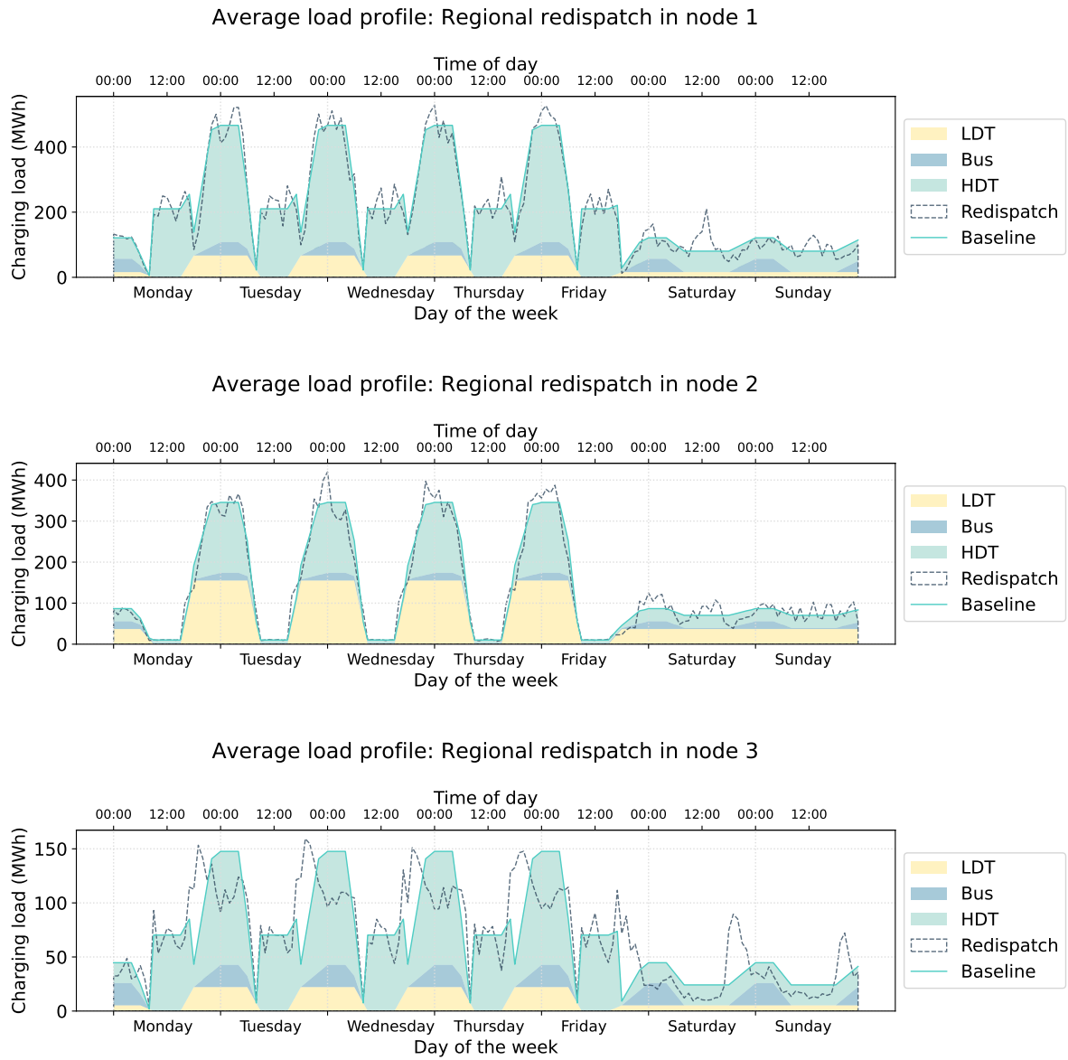
Figure E.5.: Average weekly charging profiles at three selected nodes for the Baseline and Redispatch case studies: Node A (Lower Austria, top), Node B (Vienna, middle), and Node C (Southern Austria, bottom).
