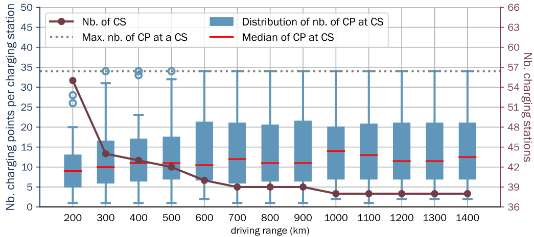
Figure 4.3.: Sensitivity analysis on driving range. Impact of the increase of the driving range of BEVs on the distribution of the number of charging points (CP) at charging stations and the total amount of charging stations (CS).
