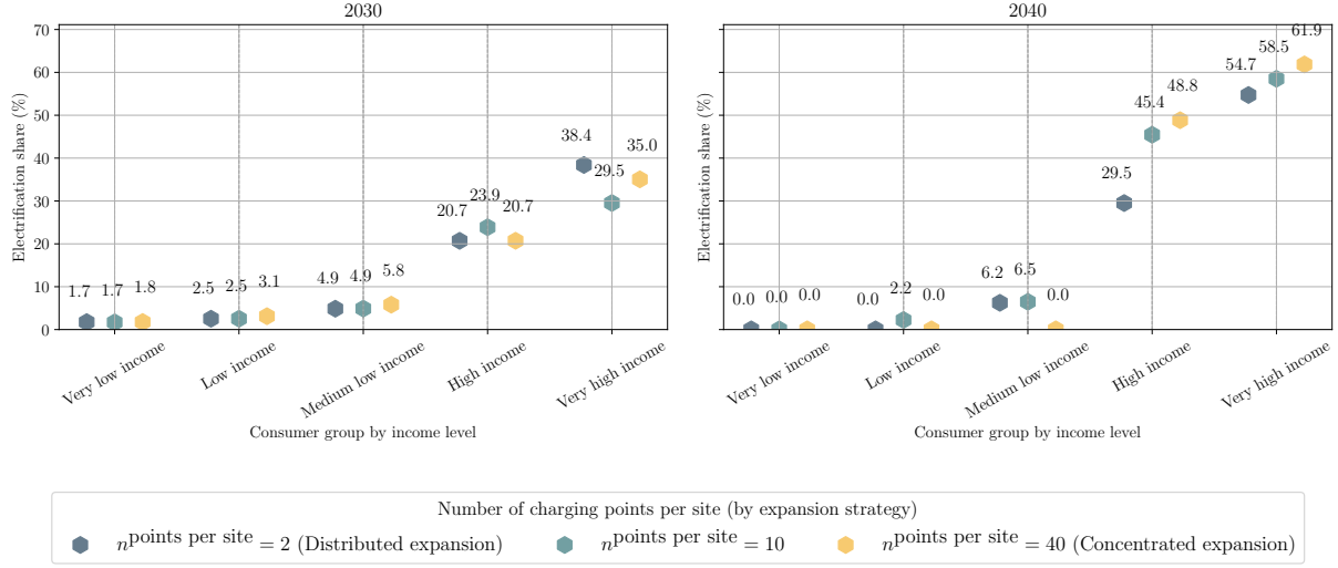
Figure 4.10.: Share of battery-electric vehicles in the passenger car fleet in 2030 and 2040 in consumer groups of different income levels for roll-out strategies of public charging infrastructure defined via the number of charging points per site ( n_{\text{points per site}} ).
