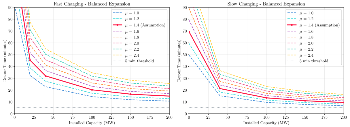
Figure C.3.: Tested detour fueling time curves for different values of circuitry \mu .
