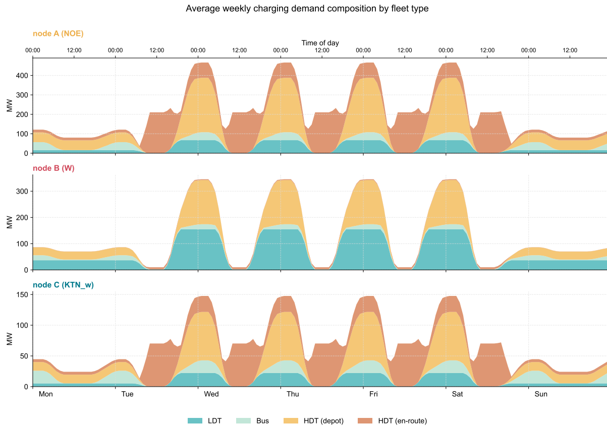
Figure 4.35.: Composition of the weekly charging demand by fleet type (light-duty trucks, heavy-duty trucks, buses) for three selected locations in Austria.
