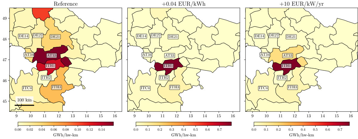
Charging demand intensity at DE-AT-IT border — 2032
