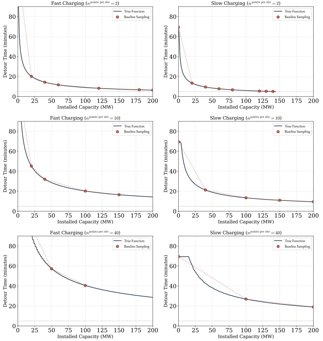
Figure C.1.: Sampling of the detour fueling time functions to introduce the relation between charging infrastructure capacity expansion and detour fueling time to the MILP.
