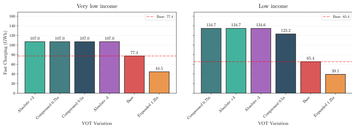
Figure C.17.: Charged energy at fast chargers by the Very low income and Low income groups in 2050 for different VoT scenarios.
