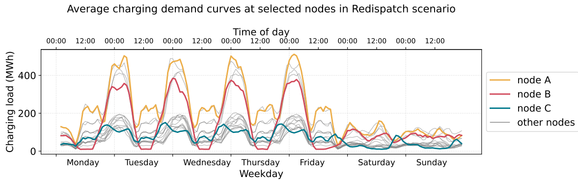
Figure E.3.: Charging load curves resulting from participation of the commercial BEV fleet in redispatch at different nodes in the Austrian transmission grid.
