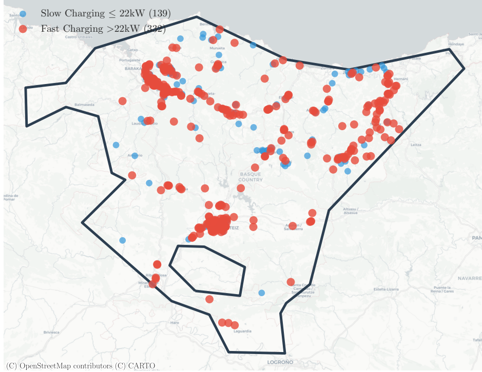
Figure C.10.: Public charger network in the Basque Country, retrieved from OpenChargeMap [216].
