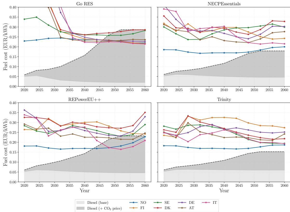
Figure 4.23.: Electricity prices (EUR/kWh) by country and GENE SYS-MOD scenario over the modelling horizon. Coloured lines show country-specific electricity prices; the light grey area shows the base diesel price and the dark grey area the diesel price including the scenario-specific carbon price component. Go RES exhibits the highest carbon price trajectory, causing diesel costs to exceed electricity prices in most countries by 2045, whereas Trinity's lower carbon prices keep diesel competitive longer.
