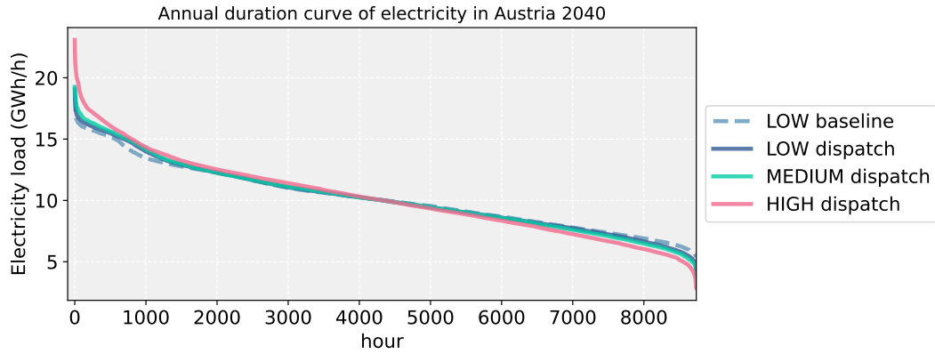
Figure E.1.: Annual duration curve of electricity demand in Austria in 2040 for different case studies and electrification scenarios.
