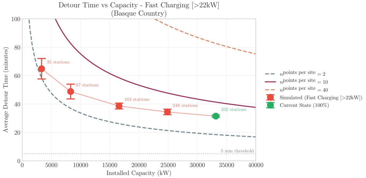
Figure C.12.: Validation of the detour fueling time function for fast chargers in the Basque Country: comparison between Monte Carlo simulation results and assumed functional form.
