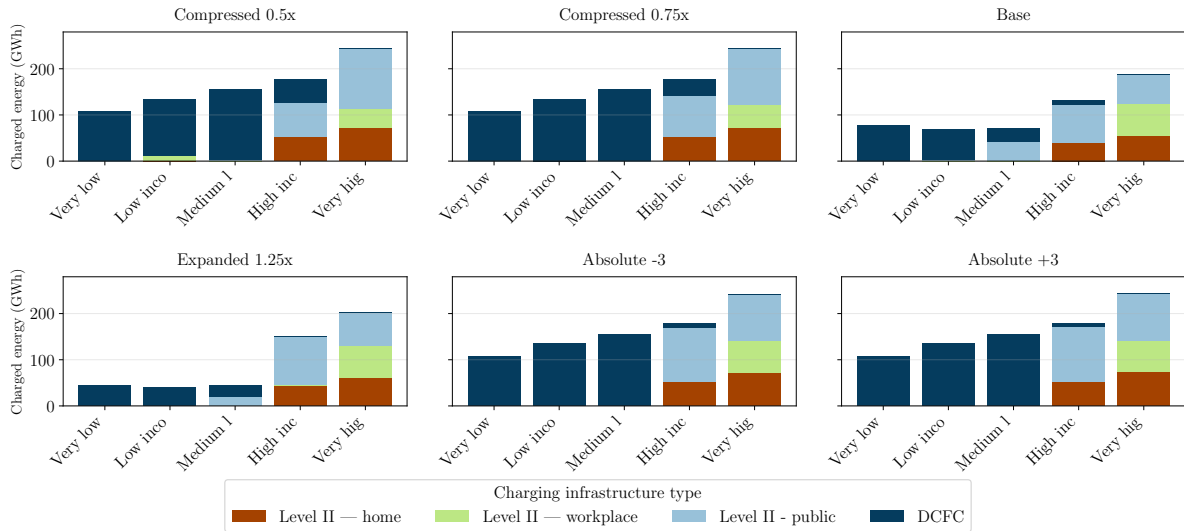
Figure C.16.: Charged energy by charger type in 2050 for different VoT scenarios.
