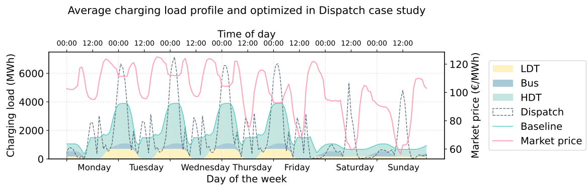
Figure 4.33.: Aggregated charging demand profile of the commercial BEV fleet in the Baseline and Dispatch case study with the average day-ahead market price.
