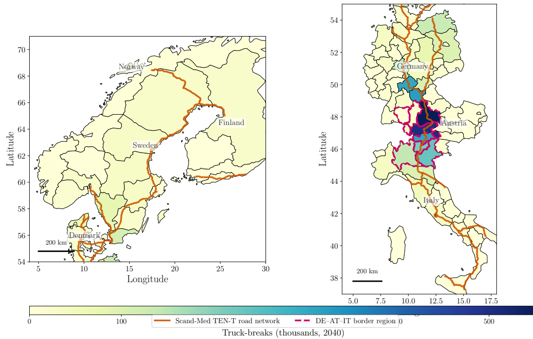
Figure 4.21.: Mandatory driver break locations per NUTS-2 region along the Scandinavian-Mediterranean corridor (2040). Orange lines show the TEN-T Scandinavian-Mediterranean road corridor geometry [180]. Colour indicates the estimated number of annual truck-breaks (thousands) at mandatory rest locations, derived from freight volumes and an average payload of 13.6 tonnes per truck. Break locations follow EU driving time regulations (45-min break after 4.5 h, 9-h rest after 9 h). Dashed magenta borders indicate the DE-AT-IT border region.
