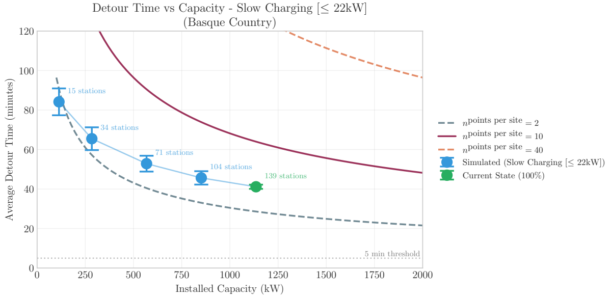
Figure C.11.: Validation of the detour fueling time function for slow chargers in the Basque Country: comparison between Monte Carlo simulation results and assumed functional form.
