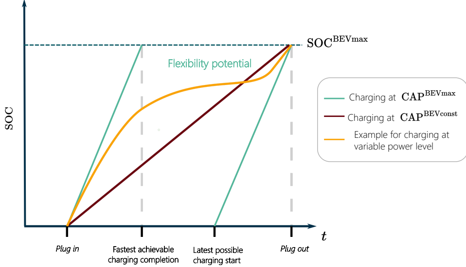
Figure 3.8.: Graphic illustration of the flexibility of a charging process
