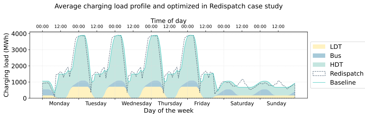
Figure E.2.: Aggregated charging demand profile of the commercial BEV fleet in the Baseline and Redispatch case studies.
