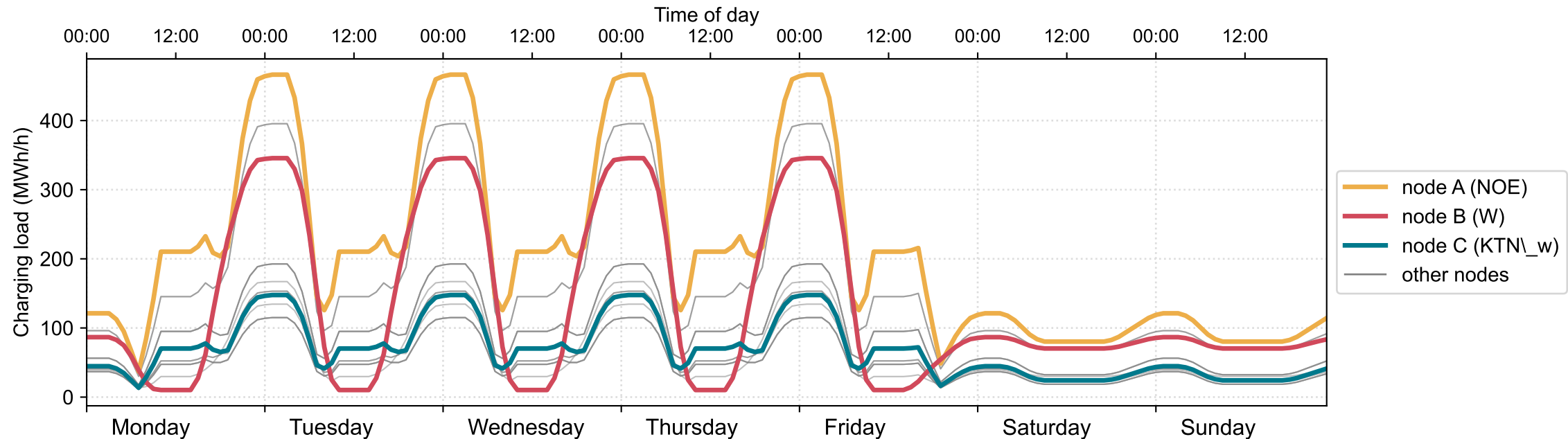
Average input charging load curves by node
