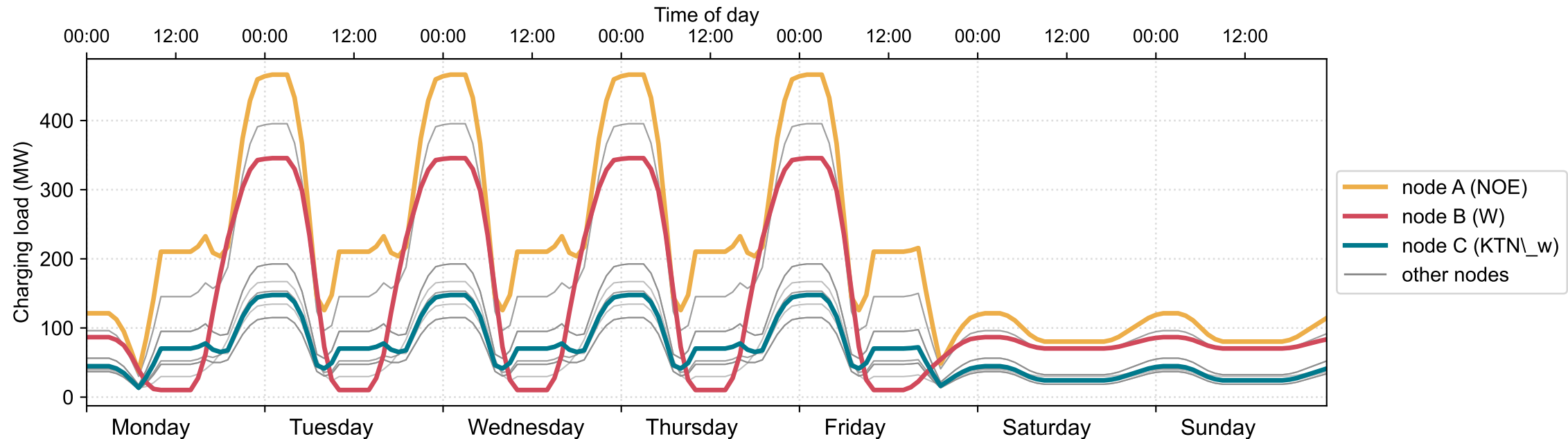
Average input charging demand curves by node
