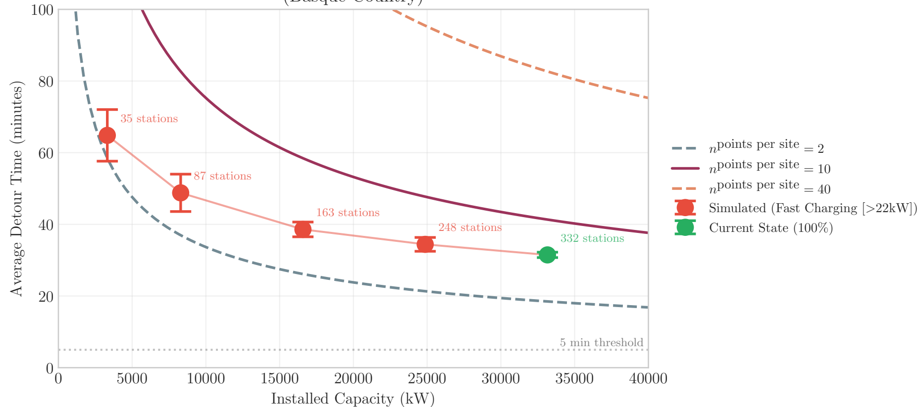
Detour Time vs Capacity - Fast Charging [ >22\text{kW} ] (Basque Country)
