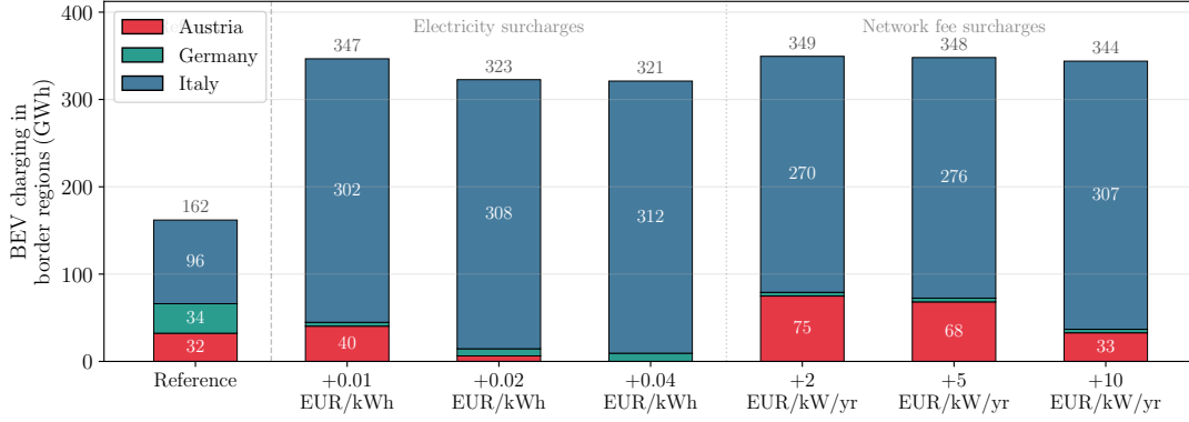
Figure 4.30.: BEV charging reallocation in the DE-AT-IT border region under Austrian electricity price and network charge locational cost premiums (2032, REPowerEU++ scenario, road-only). Stacked bars show charged energy (GWh) by country for the System-optimal (unconstrained) allocation followed by graduated premium levels.
