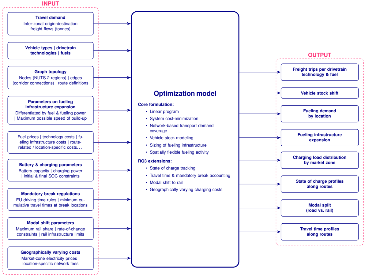
Figure 3.5.: Extended input-output relations of the optimization model for the long-distance freight transport application (RQ3), including state of charge tracking, mandatory break regulations, modal shift, and geographically varying charging costs.
