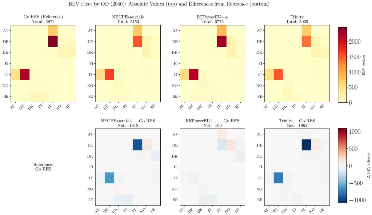
Figure 4.24.: BEV fleet by origin-destination country pair in 2040. Top row: absolute values for each scenario. Bottom row: differences relative to the Go RES reference scenario.
