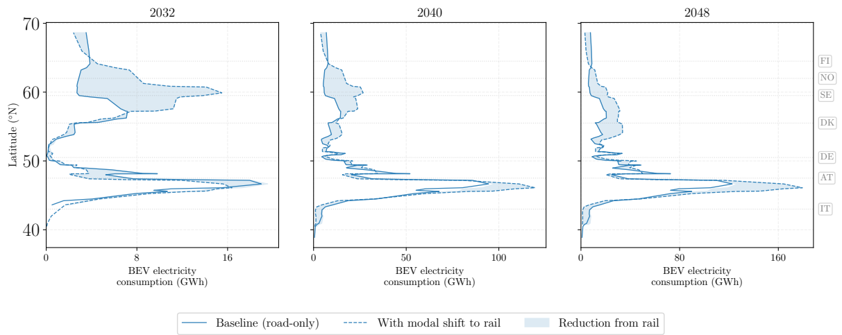
Figure 4.28.: BET electricity consumption by latitude for the Go RES scenario in 2032, 2040, and 2048. Solid line: road-only baseline; dashed line: with modal shift to rail. The shaded area indicates the reduction in charging demand from modal shift. Country centroids are annotated on the right.
