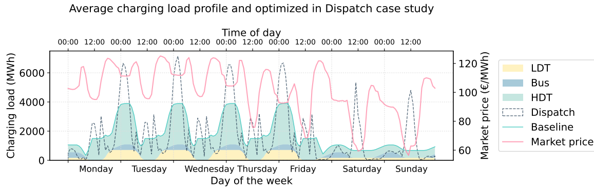
Figure 4.33.: Aggregated weekly charging demand profile of the commercial BEV fleet under baseline assumptions and with market-price-coordinated charging, together with the average day-ahead market price.
