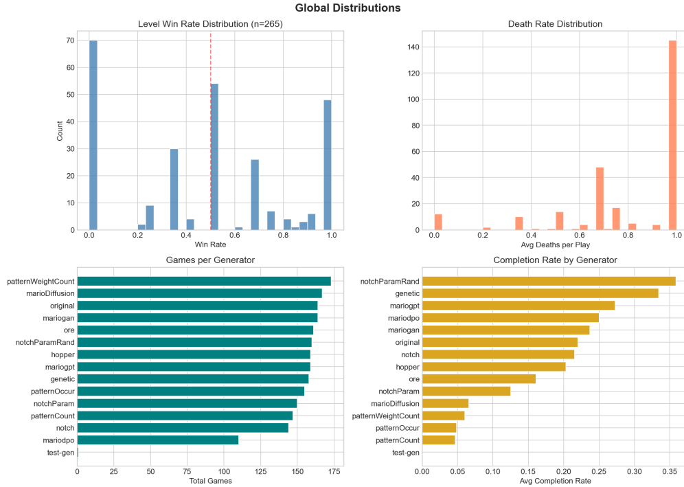
Figure 4.13: Global data distributions. Top-left: level win rate distribution centred around 0.5. Top-right: death rate distribution. Bottom: games and completion rates by generator.
