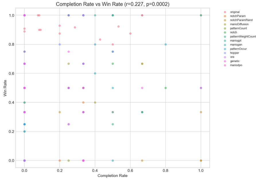
Figure 4.7: Completion rate versus win rate, coloured by generator. The significant positive correlation ( r_s = 0.227 ) indicates that playable levels are preferred.
