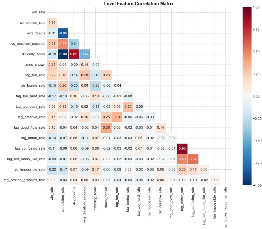
Figure 4.11: Spearman correlation matrix of level features. Win rate correlates positively with completion rate and fun-tag rate, and negatively with average deaths and too-hard-tag rate.
