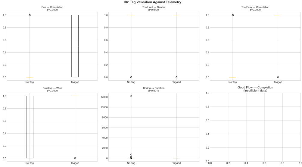
Figure 4.8: Tag validation: comparing the telemetry metric between plays tagged (right box) and not tagged (left box) with each label. All five tested associations are statistically significant.
