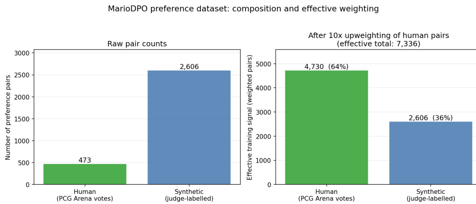
Figure 5.1: MarioDPO preference dataset: raw pair counts (left) and the same counts after applying the 10 \times upweighting of human PCG Arena pairs (right). The few hundred human comparisons contribute roughly two thirds of the effective training signal, while pairs labelled by the judge function (Section ??) primarily broaden coverage.
