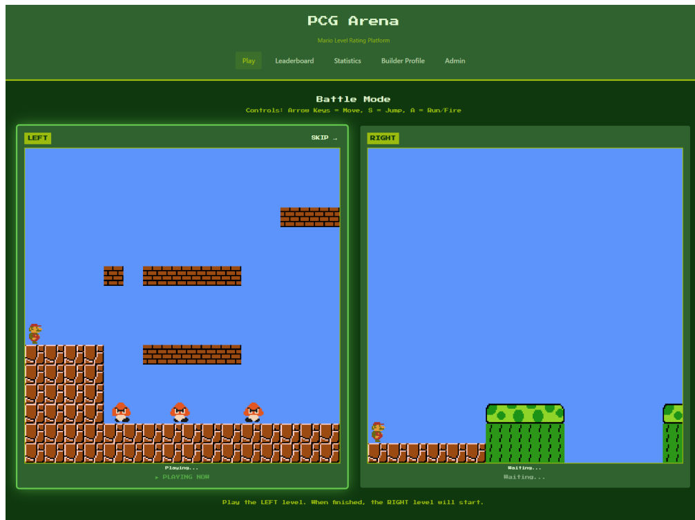
Figure 3.2: Main gameplay view: the player experiences a procedurally generated level in the browser-based Mario engine.
