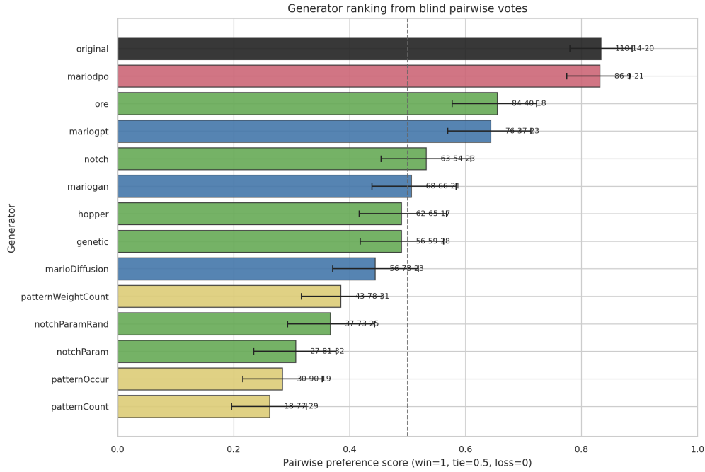
Figure 4.2: Generator ranking from blind pairwise votes. Bars show mean preference score, where win = 1, tie = 0.5, and loss = 0; horizontal intervals show bootstrap uncertainty. The text at the end of each bar gives the win-loss-tie record.
