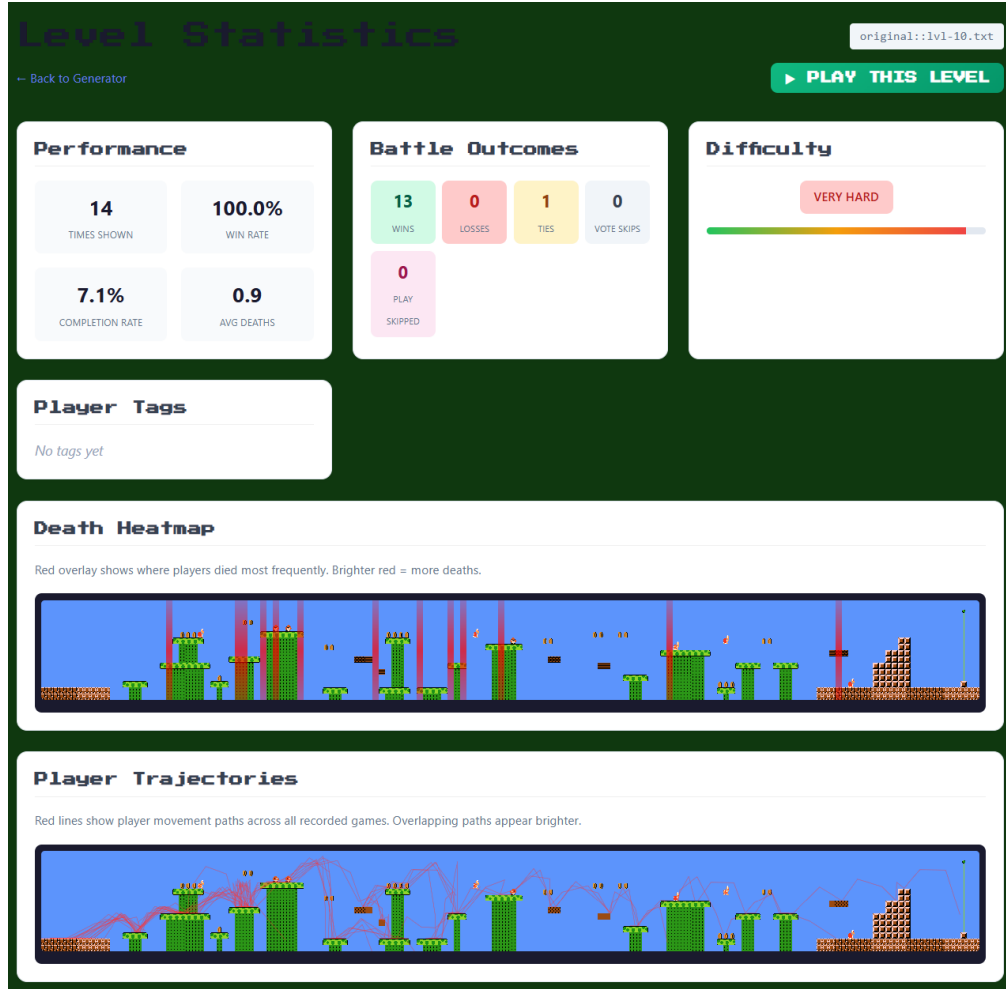
Figure 4.9: Detailed Level Statistics page from PCG Arena. The interface supports qualitative inspection of individual levels through trajectory overlays, death locations, tag counts, and level visualization.
