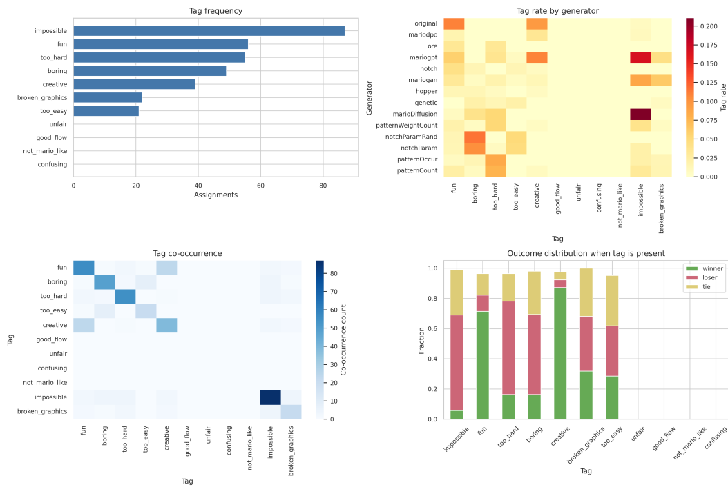
Figure 4.12: Tag semantics summary. The panels show tag frequency, tag rate by generator, tag co-occurrence, and the outcome distribution for tagged sides.
