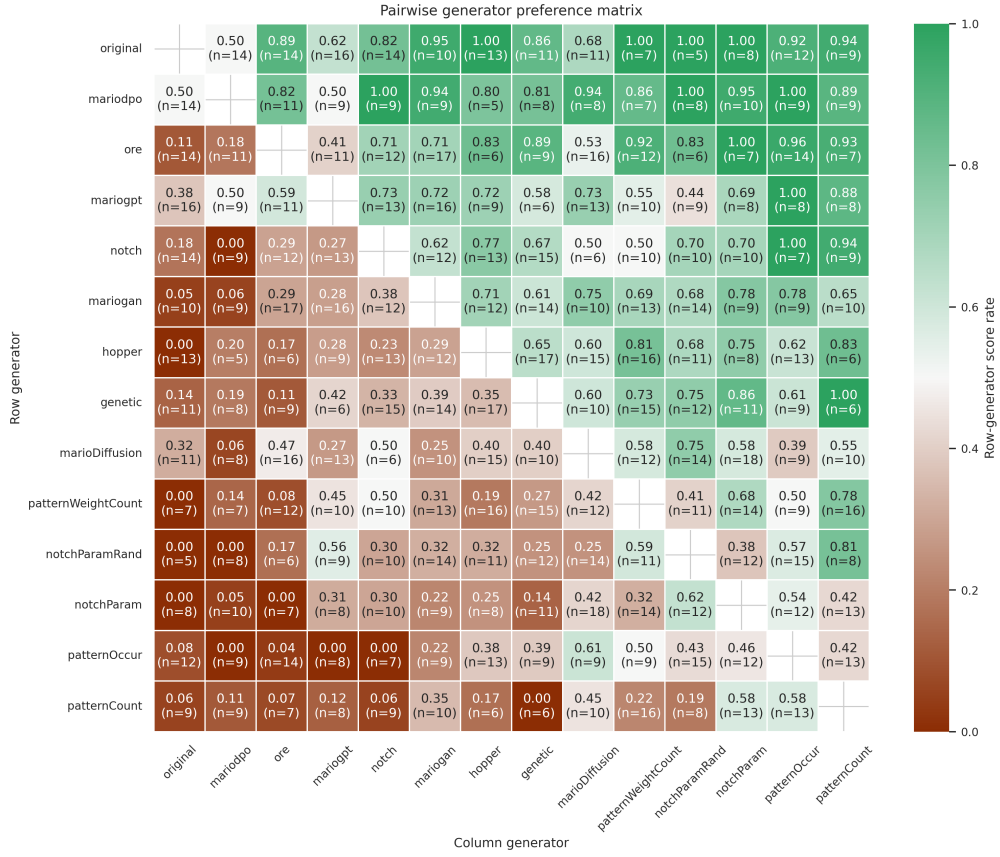
Figure 4.3: Pairwise generator preference matrix ordered by overall ranking. Each cell is the score rate for the row generator against the column generator, with ties counted as 0.5. Green indicates a higher score rate for the row generator.
