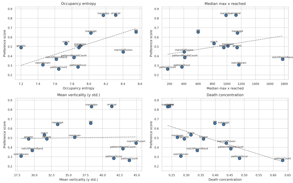
Figure 4.8: Trajectory-derived behavioral summaries versus generator preference score. Higher occupancy entropy and lower death concentration are associated with stronger generators in this export.
