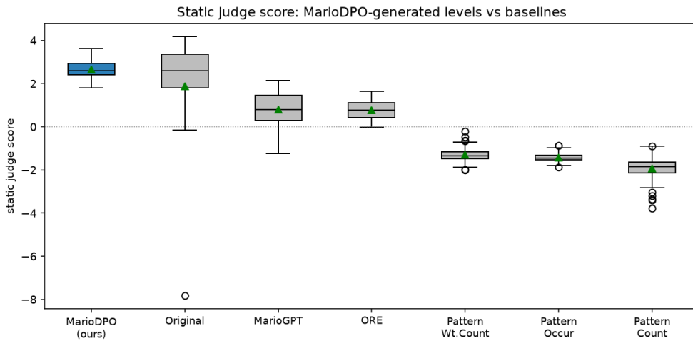
Figure 5.2: Static judge scores of MarioDPO-generated levels against the baseline generators (green triangles mark means). The generated levels sit at the top of the distribution, matching the hand-authored original corpus and clearly exceeding the other procedural generators.
