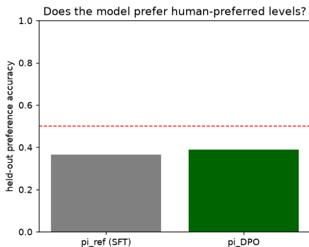
Figure 5.3: Held-out preference accuracy: how often each policy assigns higher likelihood to the human-preferred level. DPO improves over its SFT reference; the dashed line marks chance. Absolute values are modest because length-normalised sequence likelihood over a short window is a strict proxy on a small split.
