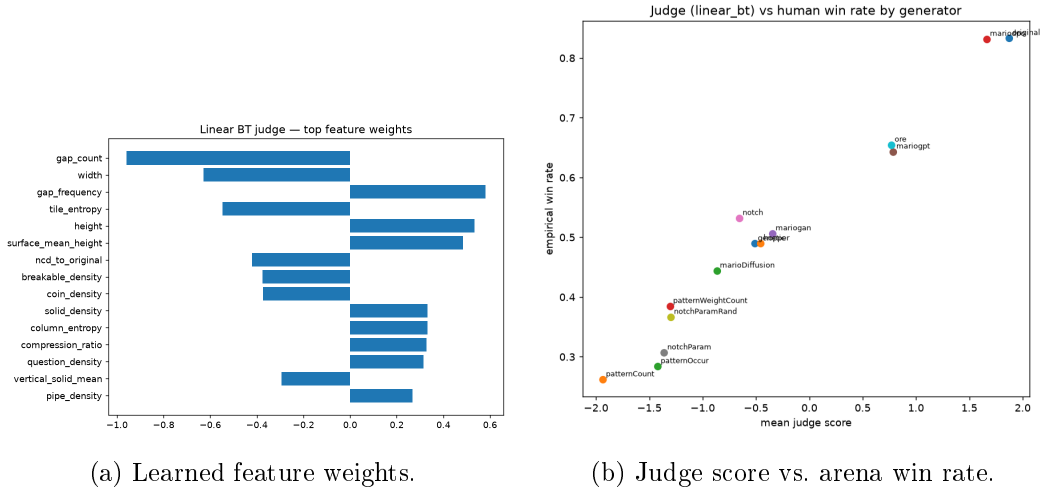
Figure 5.1: Judge-function validation. (a) The linear Bradley–Terry judge penalises gaps and excess width while rewarding structural variety and reward content. (b) Aggregated per generator, the judge score tracks the empirical human win rate ( r_s = 0.965 ), recovering almost the entire arena leaderboard from static features alone.
