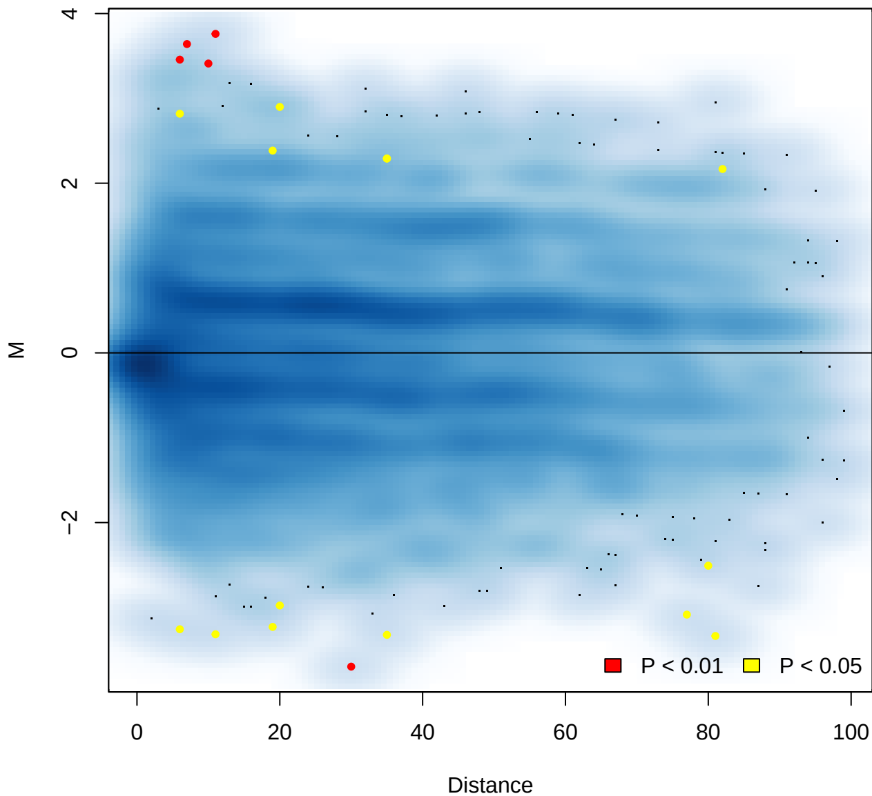
MD Plot
