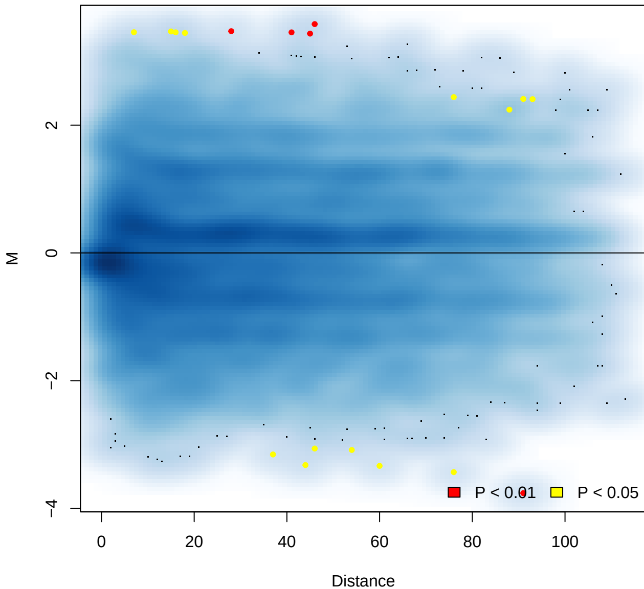
MD Plot
