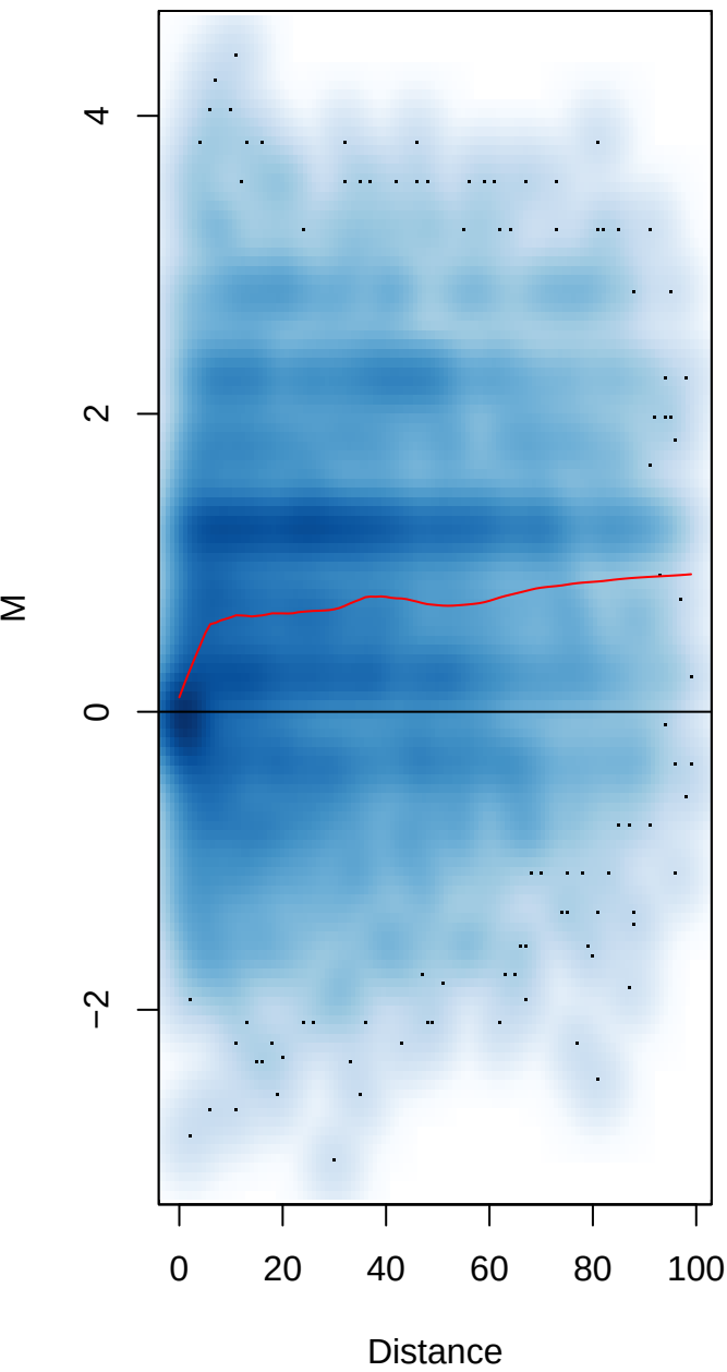
Before loess
