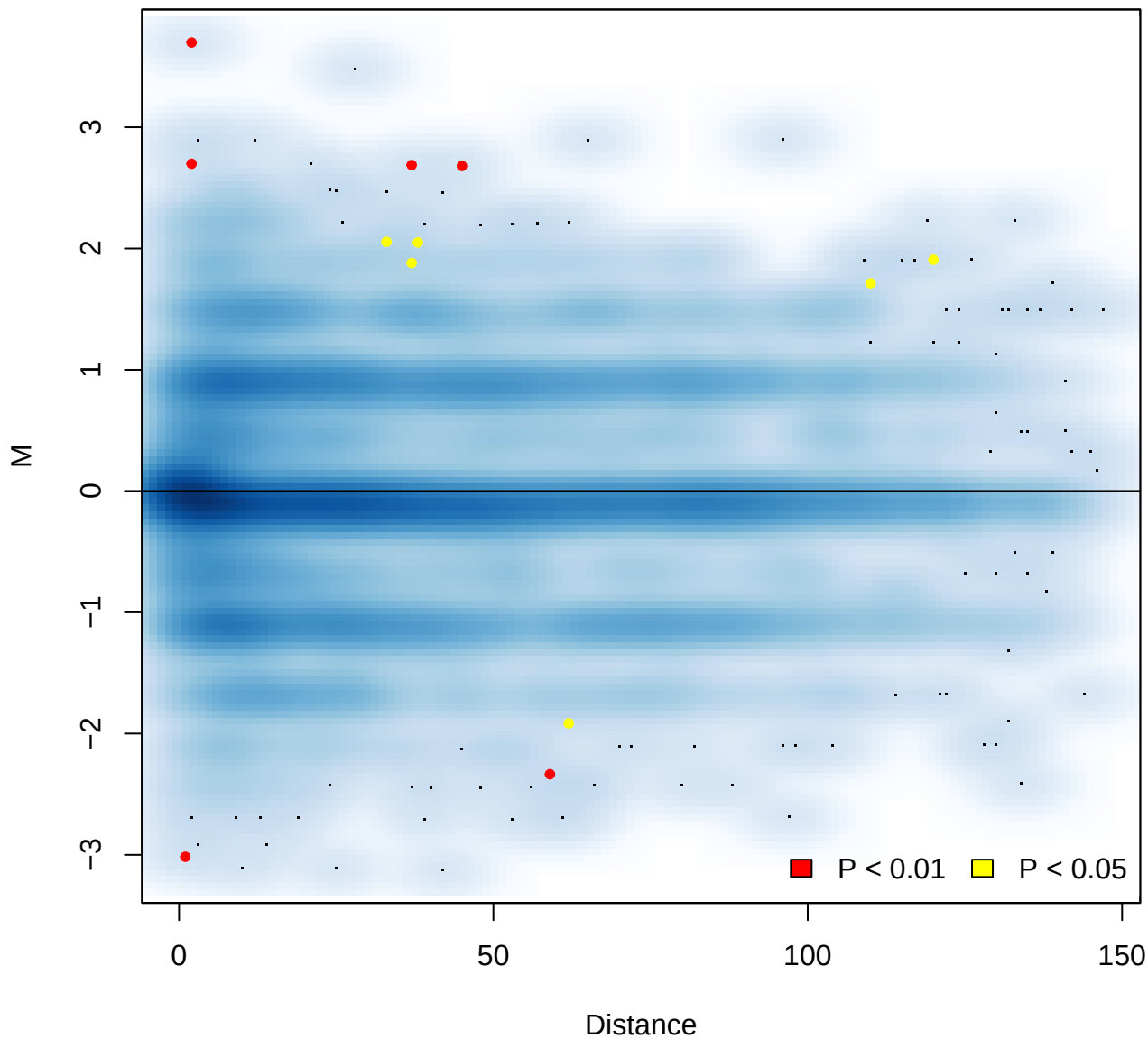
MD Plot
