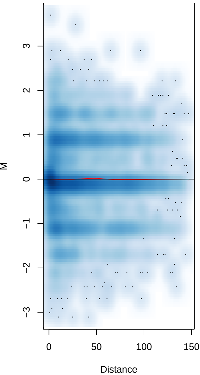
Before loess
