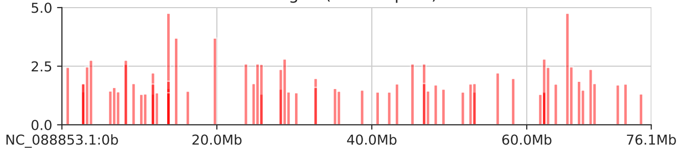
signif (HiCcompare)
