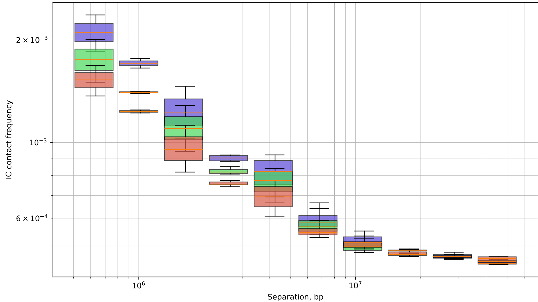
250kb - chr3, (10 bins)
