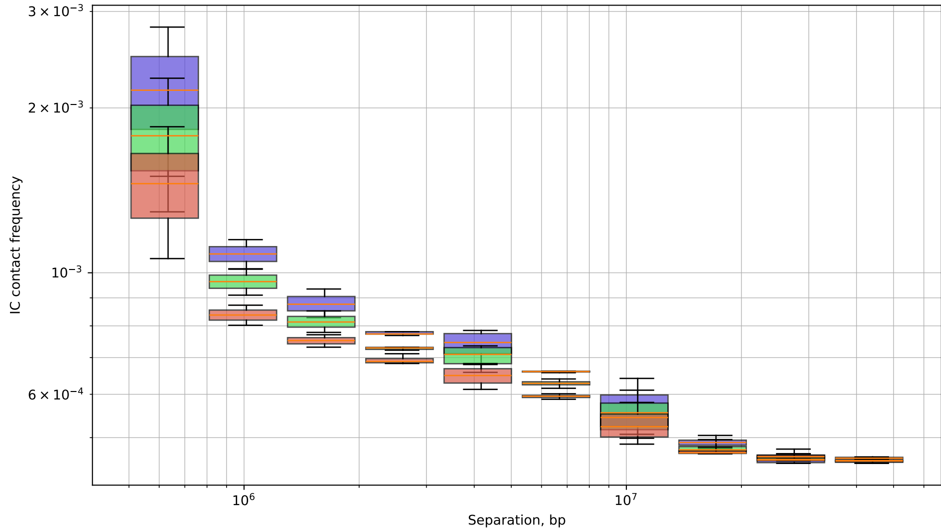
250kb - chr1, (10 bins)
