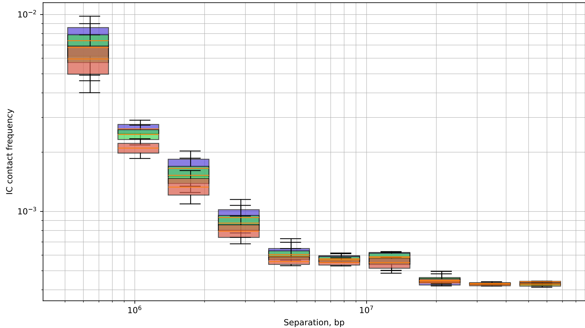
250kb - chr5, (10 bins)
