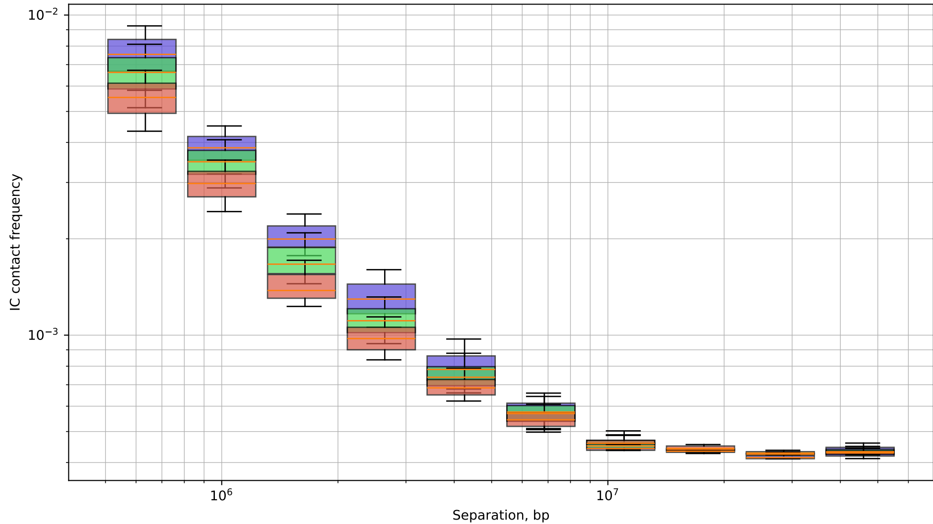
250kb - chr8, (10 bins)
