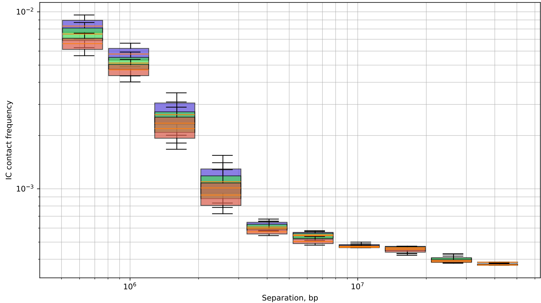
250kb - chr4, (10 bins)
