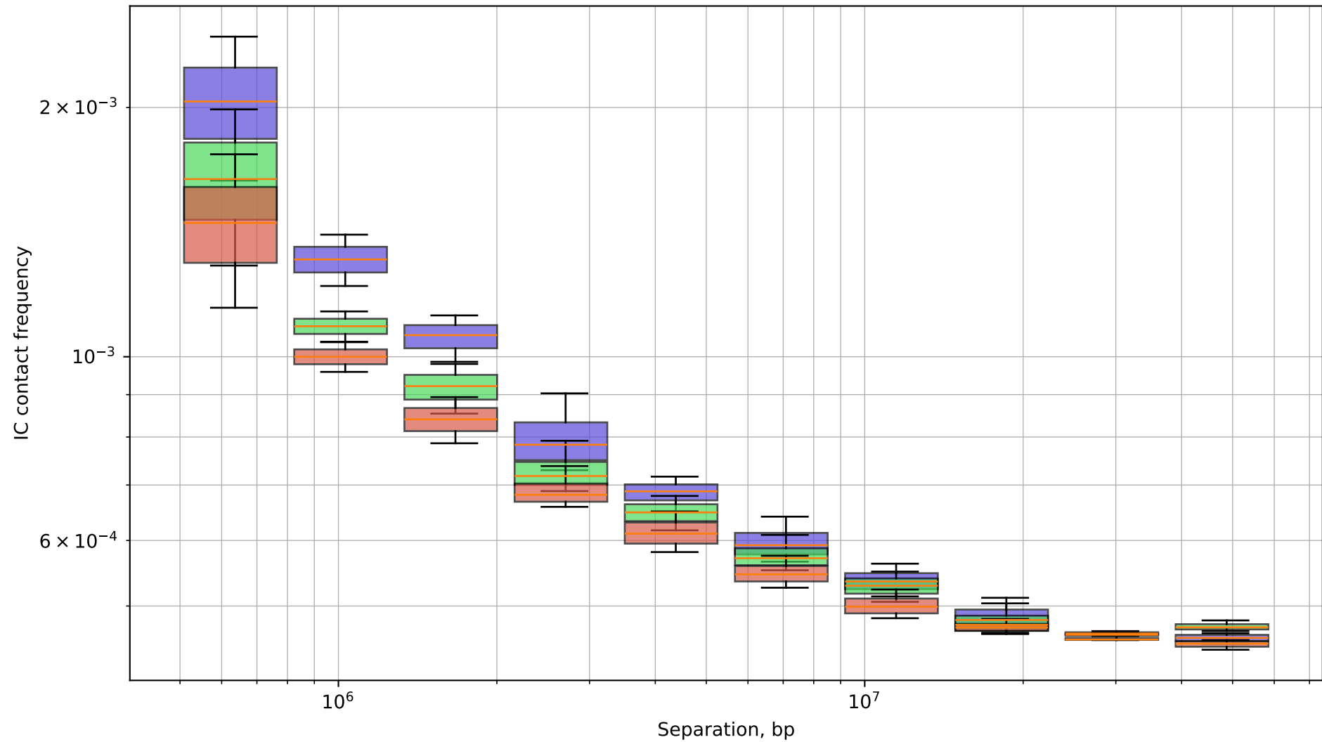
250kb - chr7, (10 bins)
