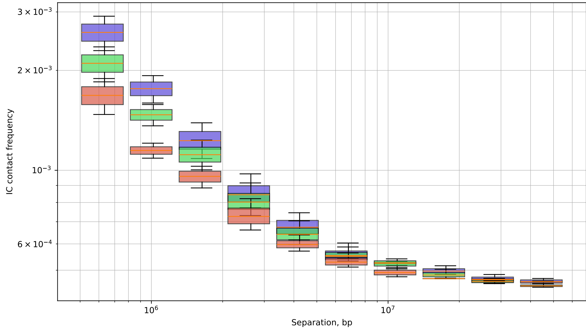
250kb - chr10, (10 bins)
