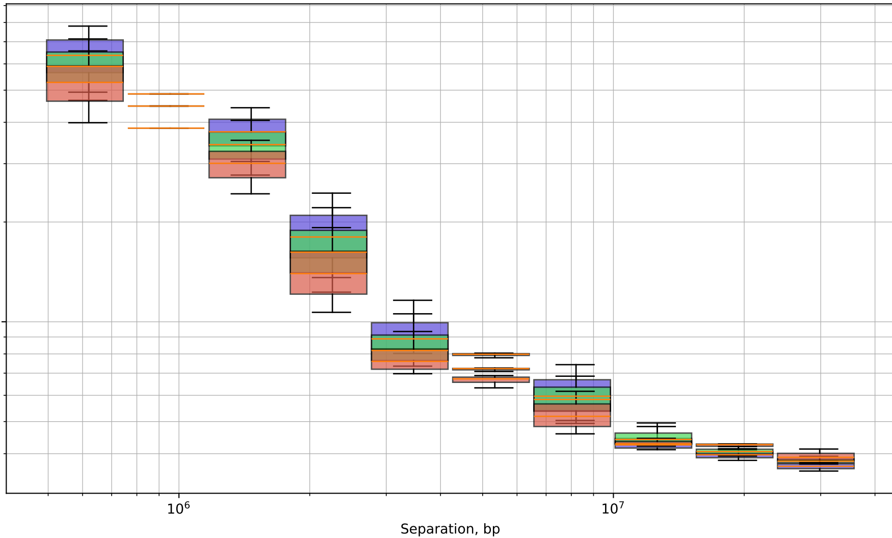
250kb - chr9, (10 bins)
