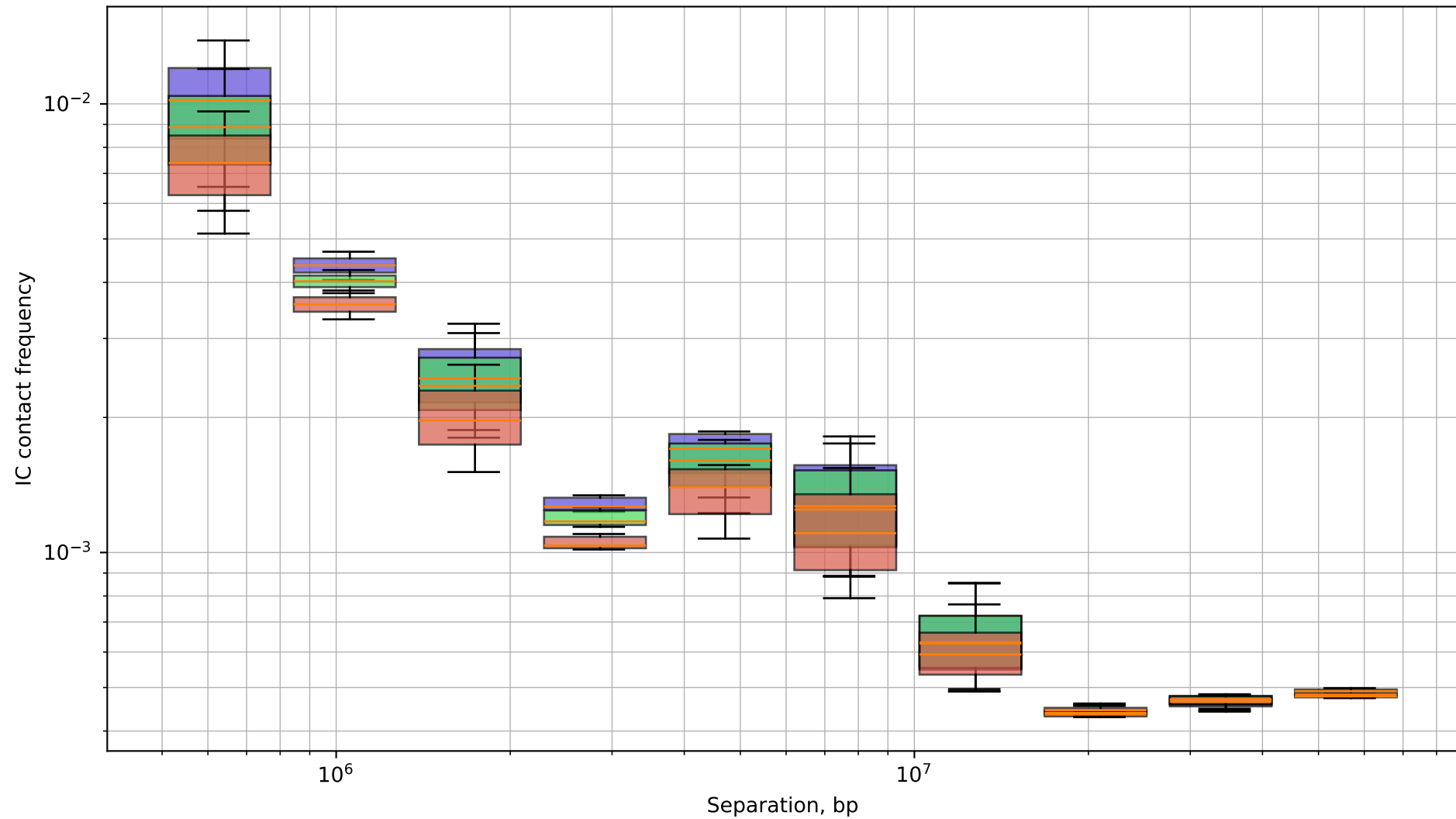
250kb - chr2, (10 bins)
