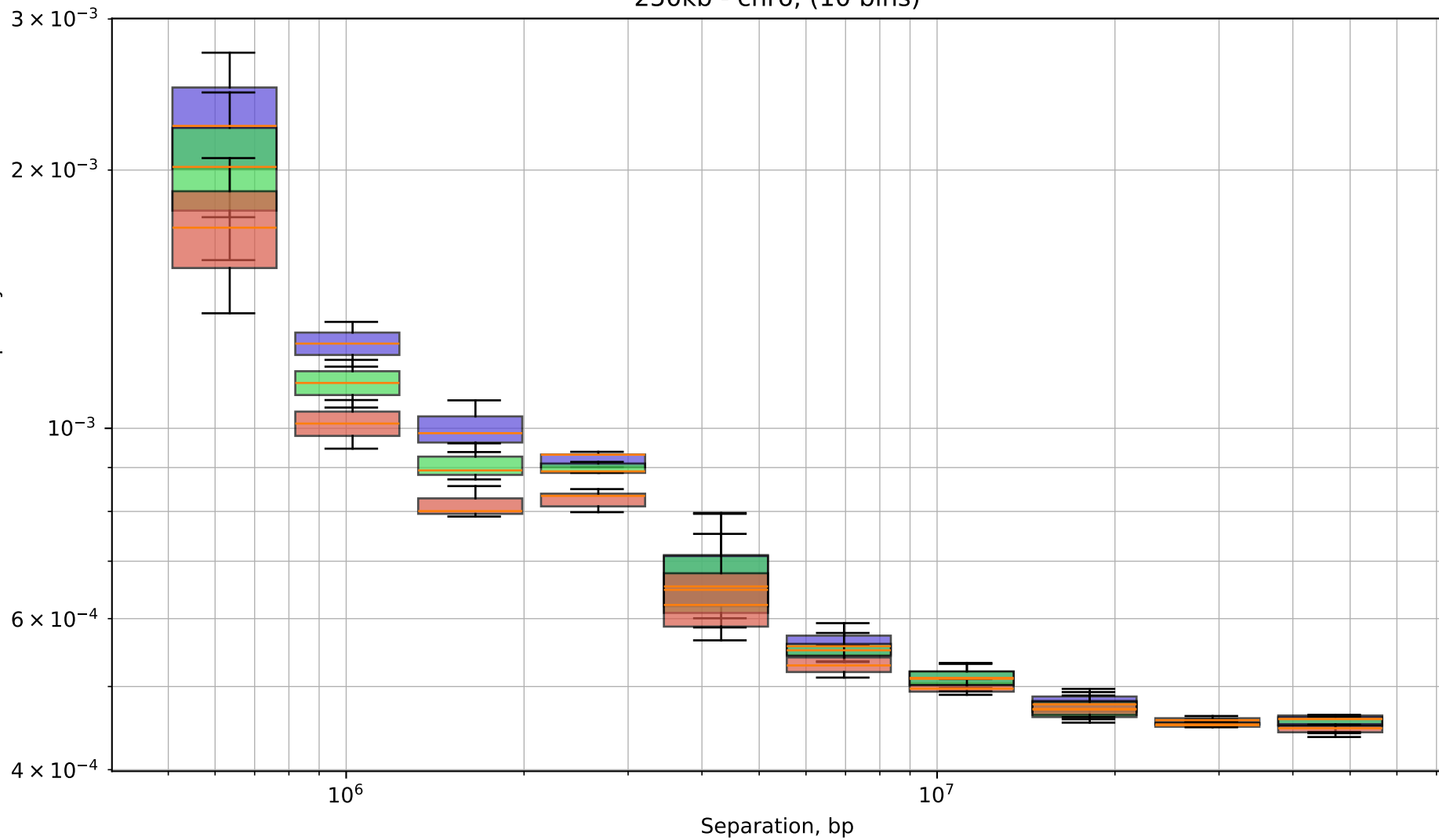
250kb - chr6, (10 bins)
