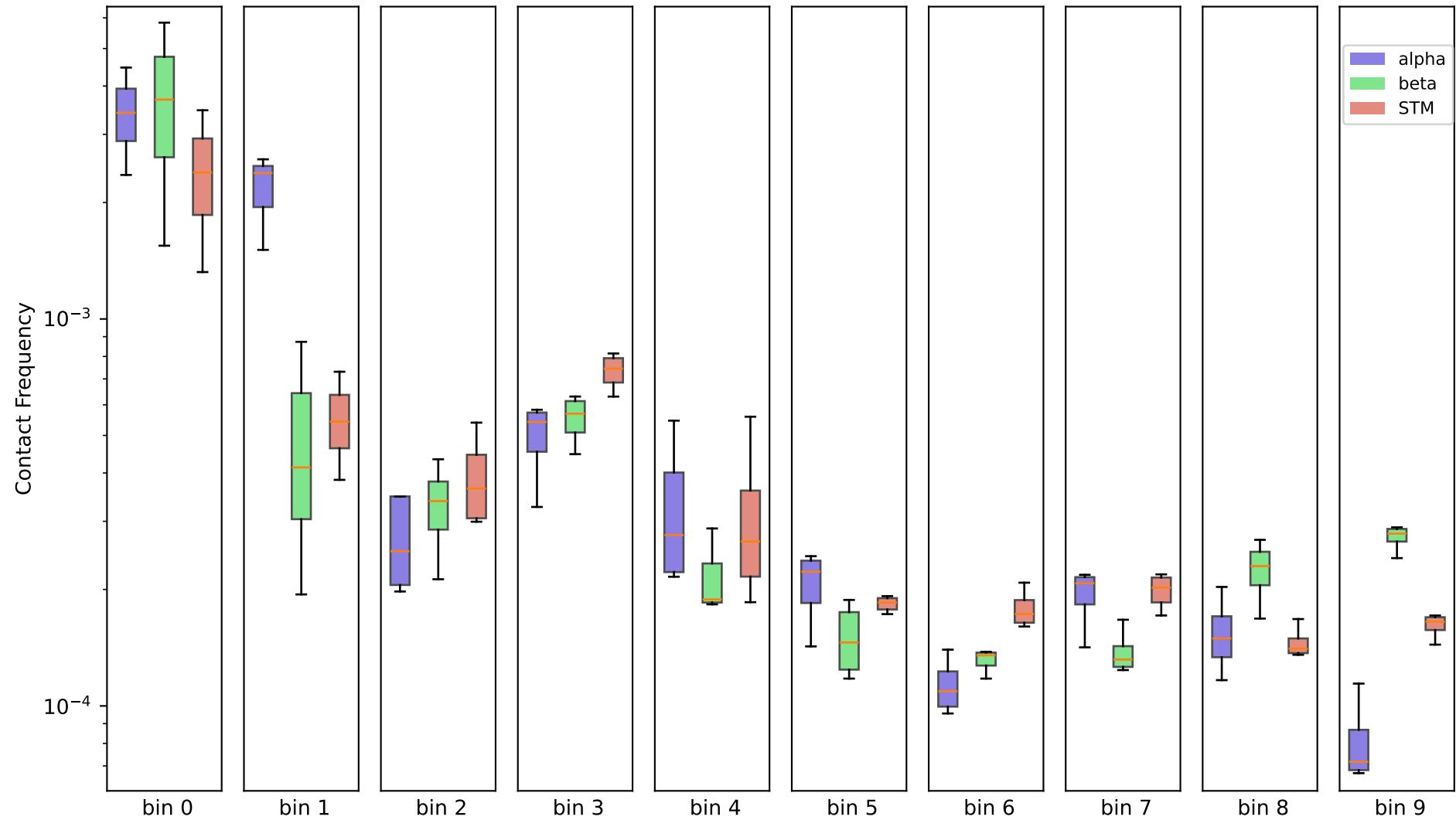
100kb - chr7, (10 bins) - 50k contacts per sample
