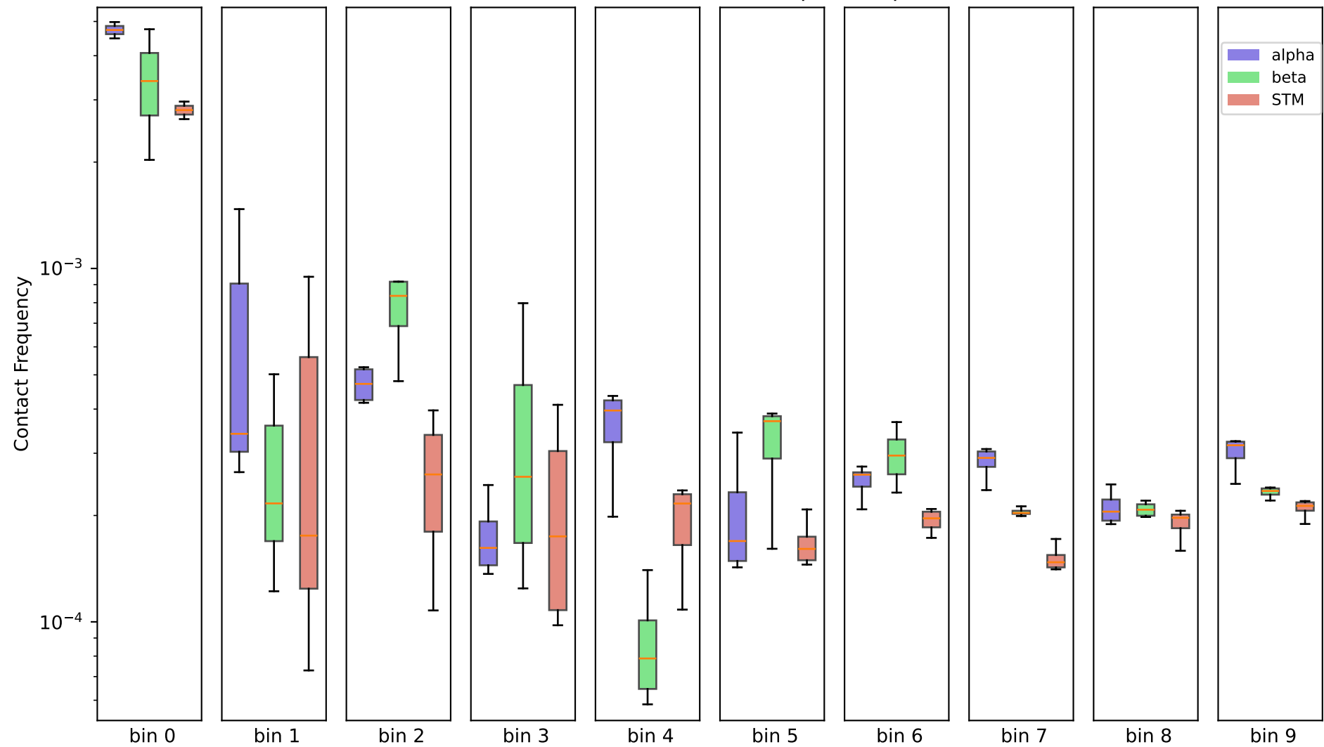
100kb - chr1, (10 bins) - 50k contacts per sample
