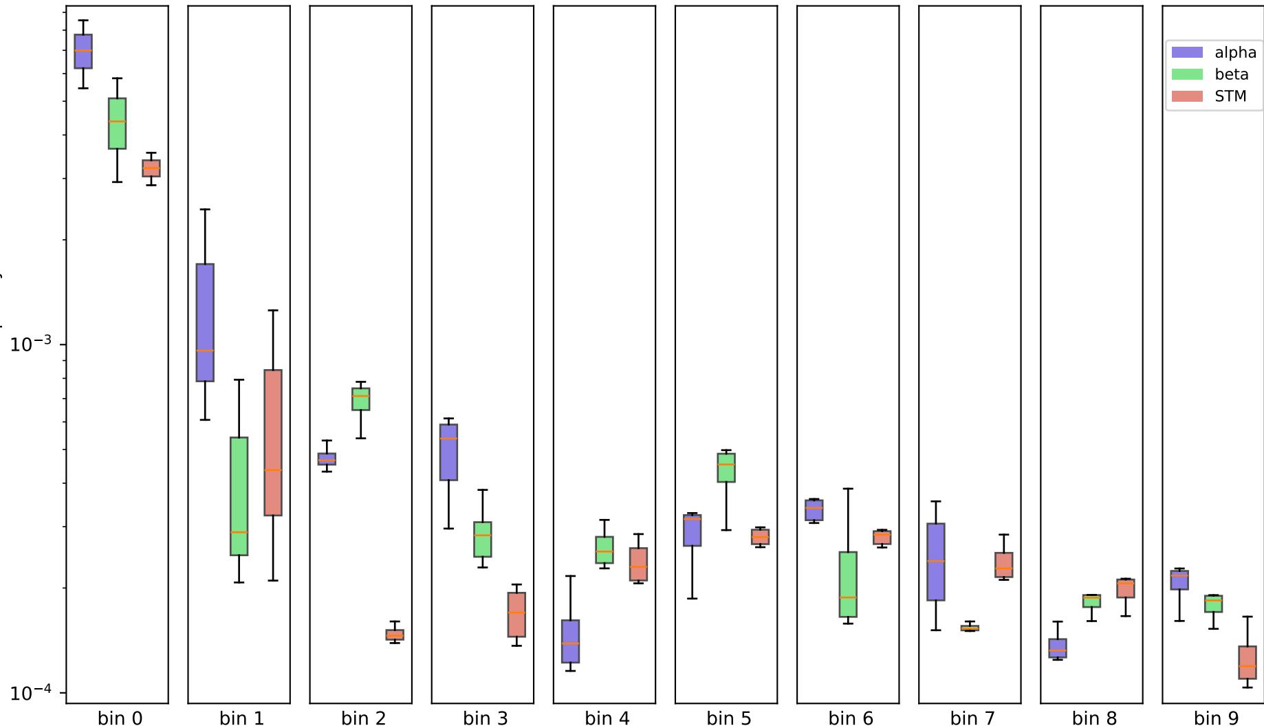
100kb - chr10, (10 bins) - 50k contacts per sample
