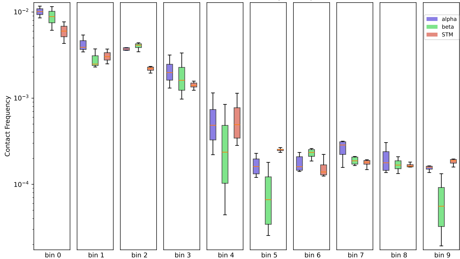
100kb - chr4, (10 bins) - 50k contacts per sample
