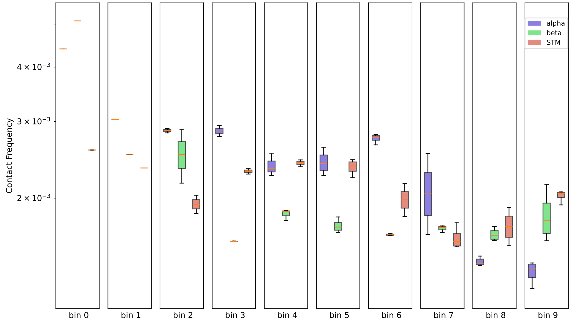
1Mb - chr3, (10 bins) - 50k contacts per sample
