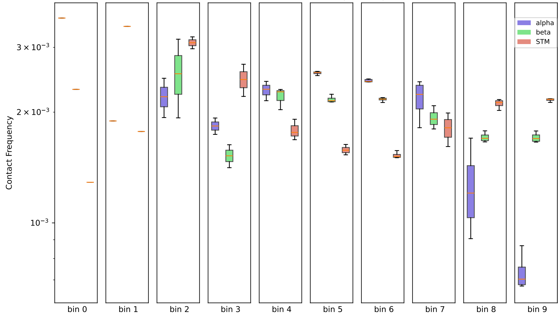
1Mb - chr10, (10 bins) - 50k contacts per sample
