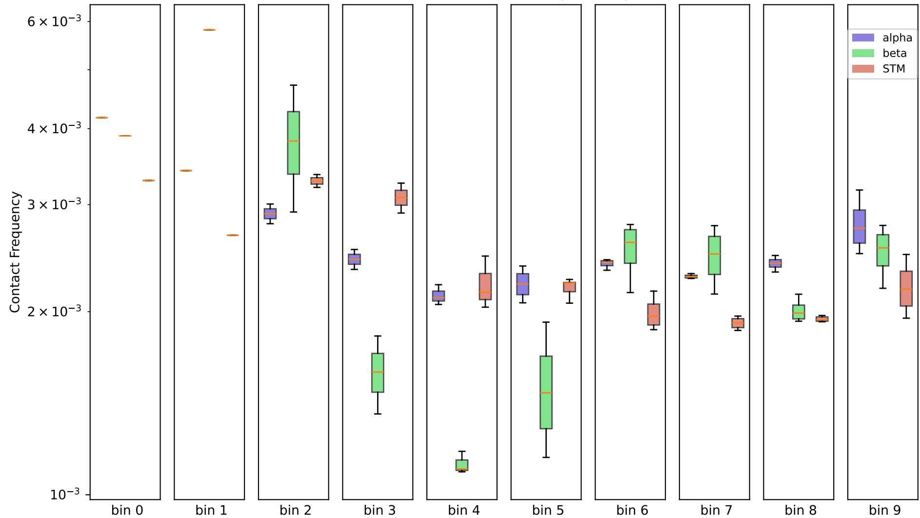
1Mb - chr8, (10 bins) - 50k contacts per sample
