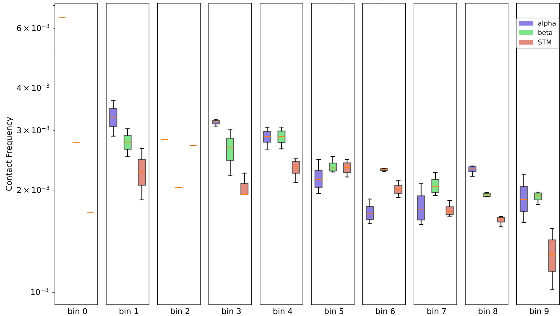
1Mb - chr5, (10 bins) - 50k contacts per sample
