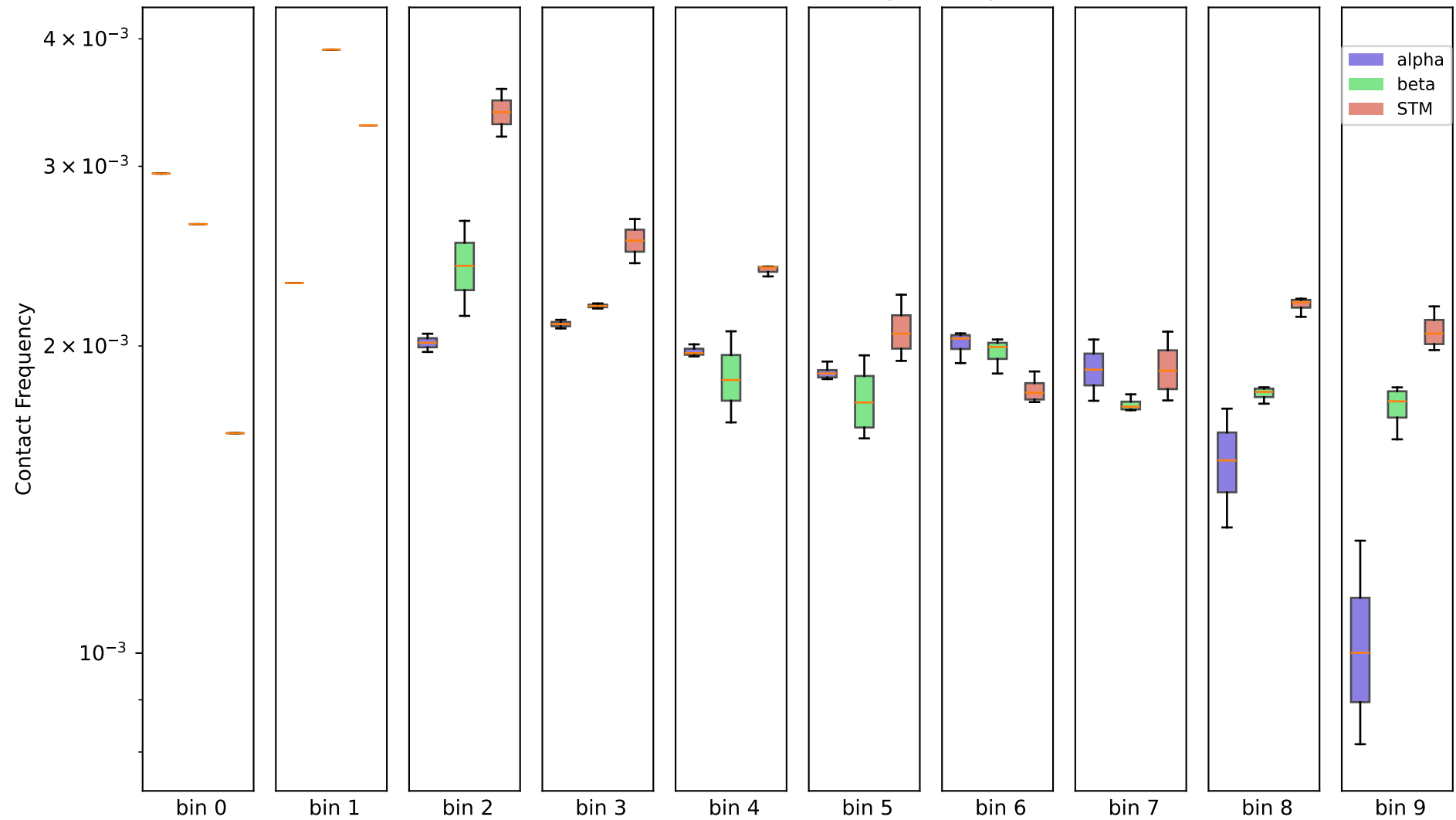
1Mb - chr6, (10 bins) - 50k contacts per sample
