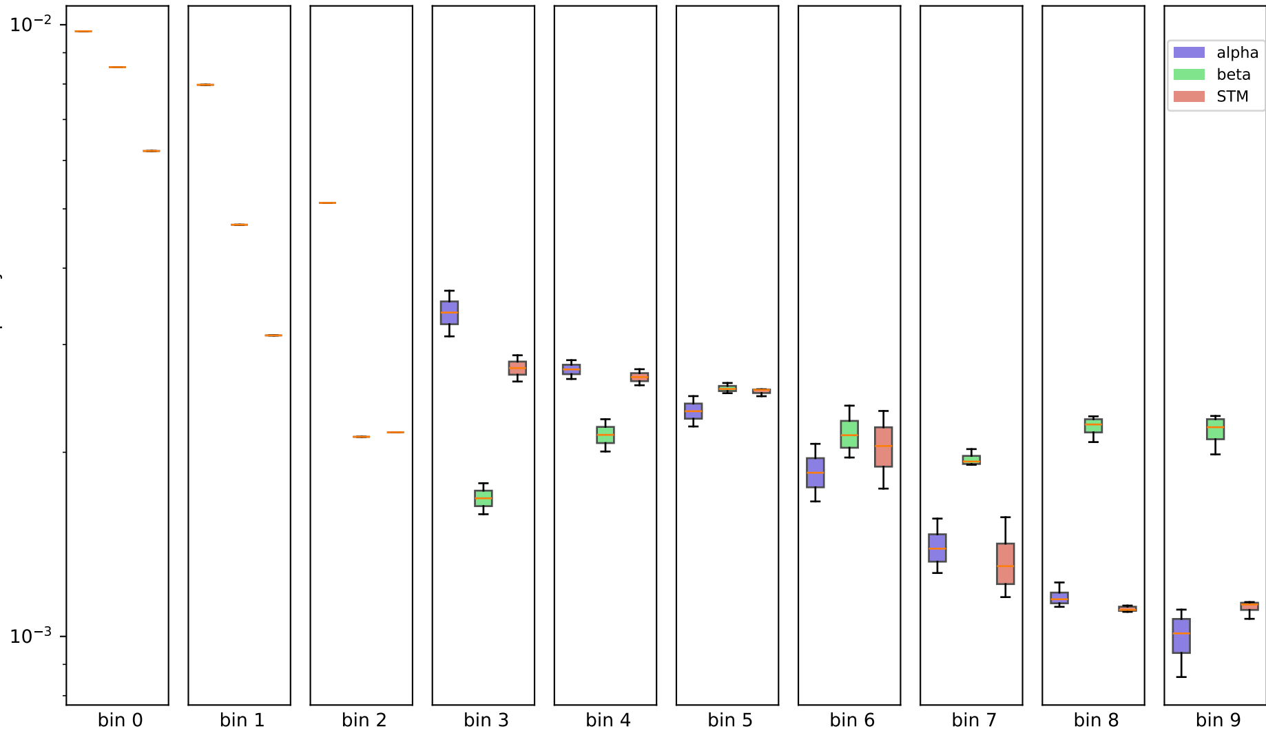
1Mb - chr9, (10 bins) - 50k contacts per sample
