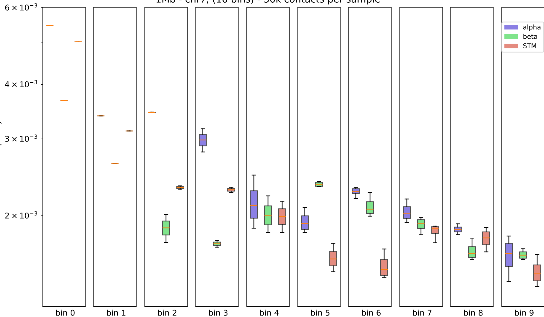
1Mb - chr7, (10 bins) - 50k contacts per sample
