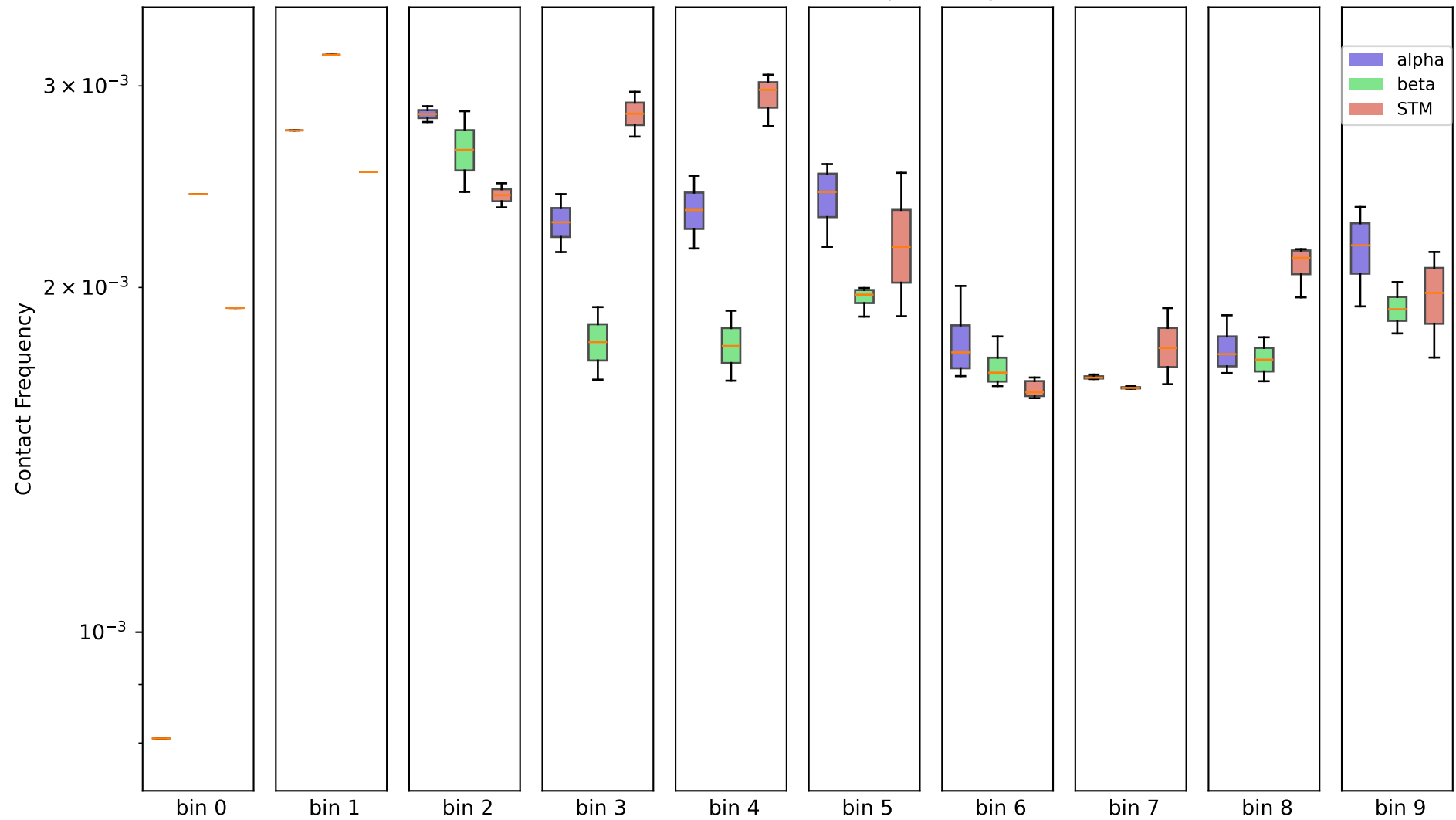
1Mb - chr1, (10 bins) - 50k contacts per sample
