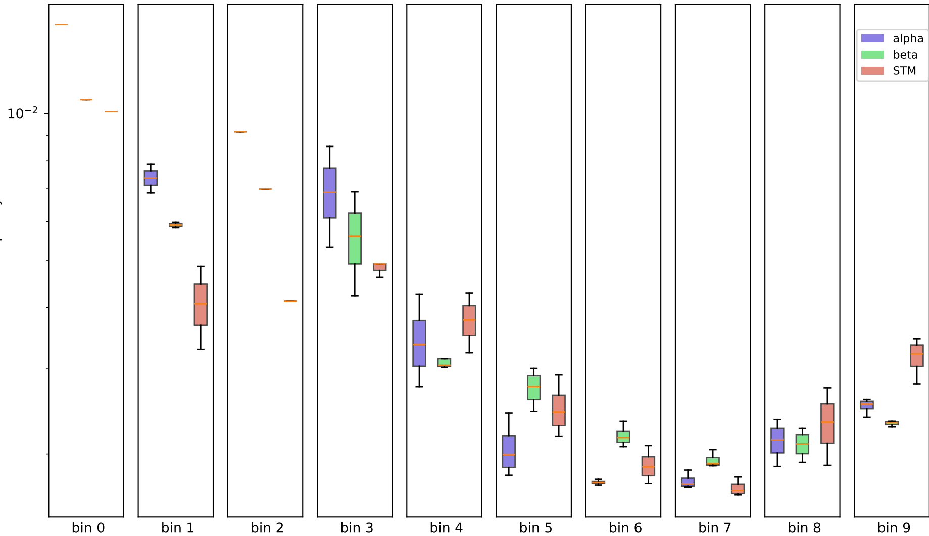
1Mb - chr2, (10 bins) - 50k contacts per sample
