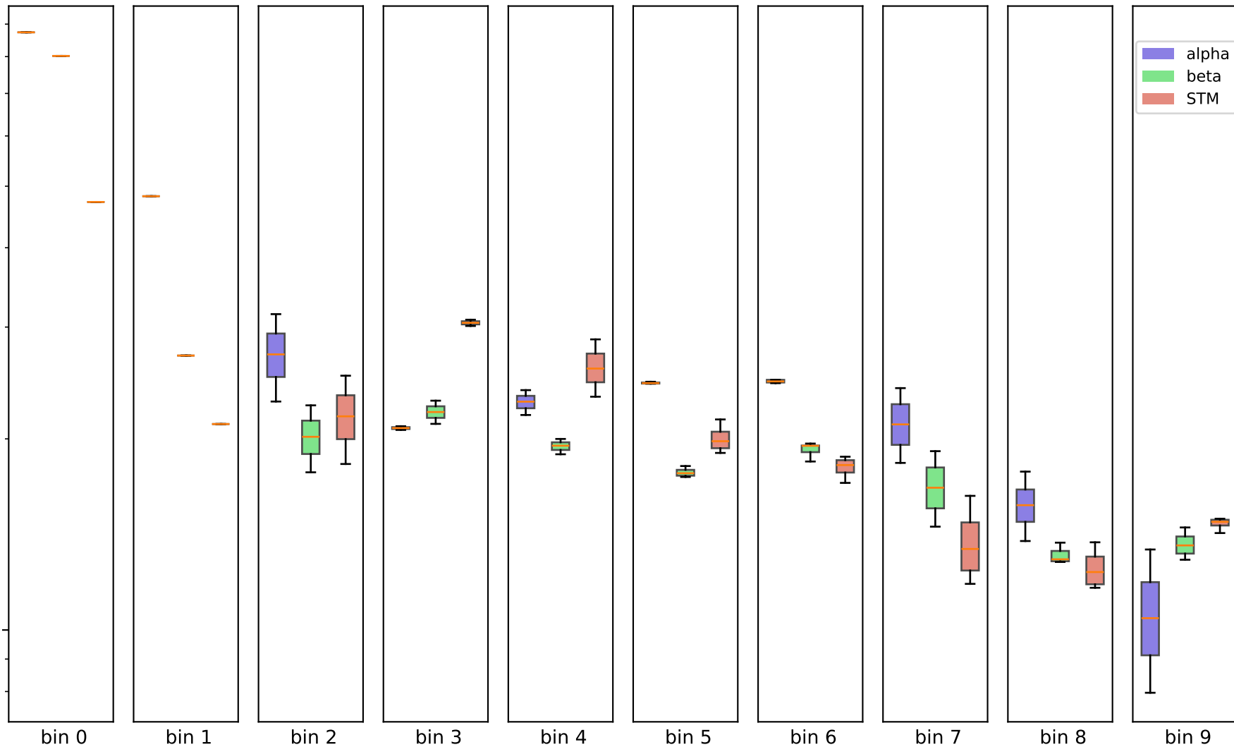
1Mb - chr4, (10 bins) - 50k contacts per sample
