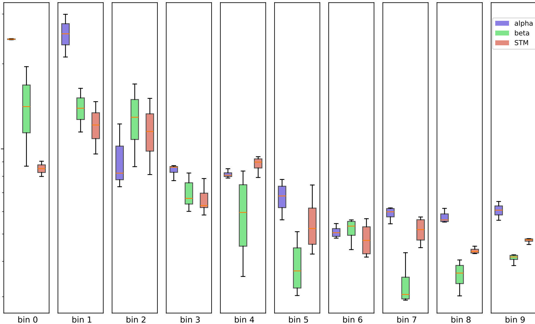
250kb - chr3, (10 bins) - 50k contacts per sample
