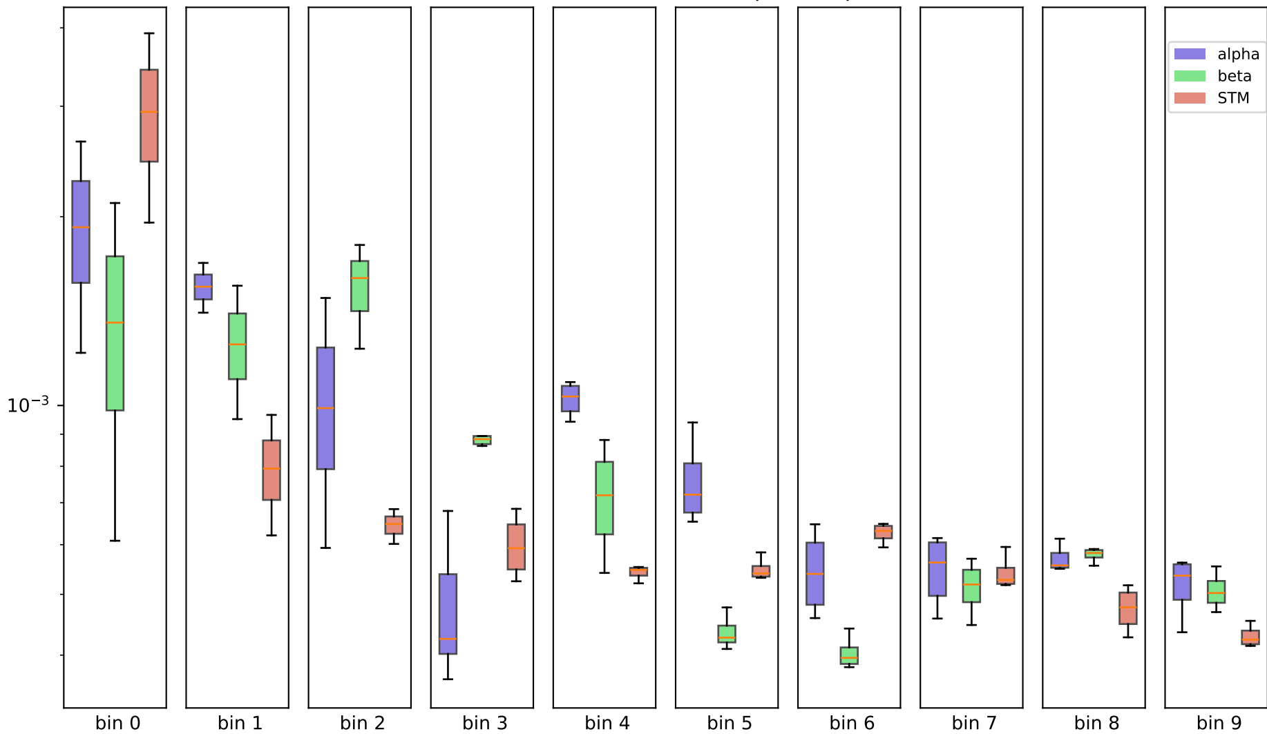
250kb - chr1, (10 bins) - 50k contacts per sample
