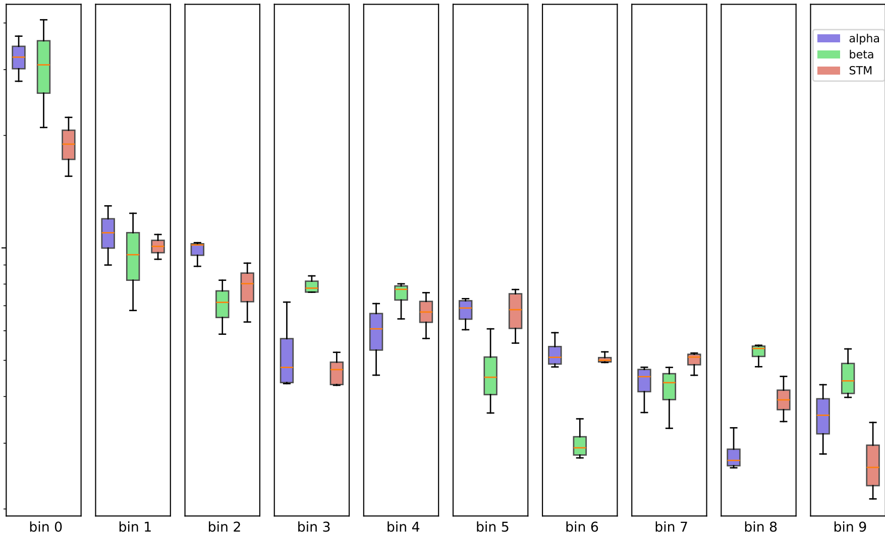
250kb - chr7, (10 bins) - 50k contacts per sample
