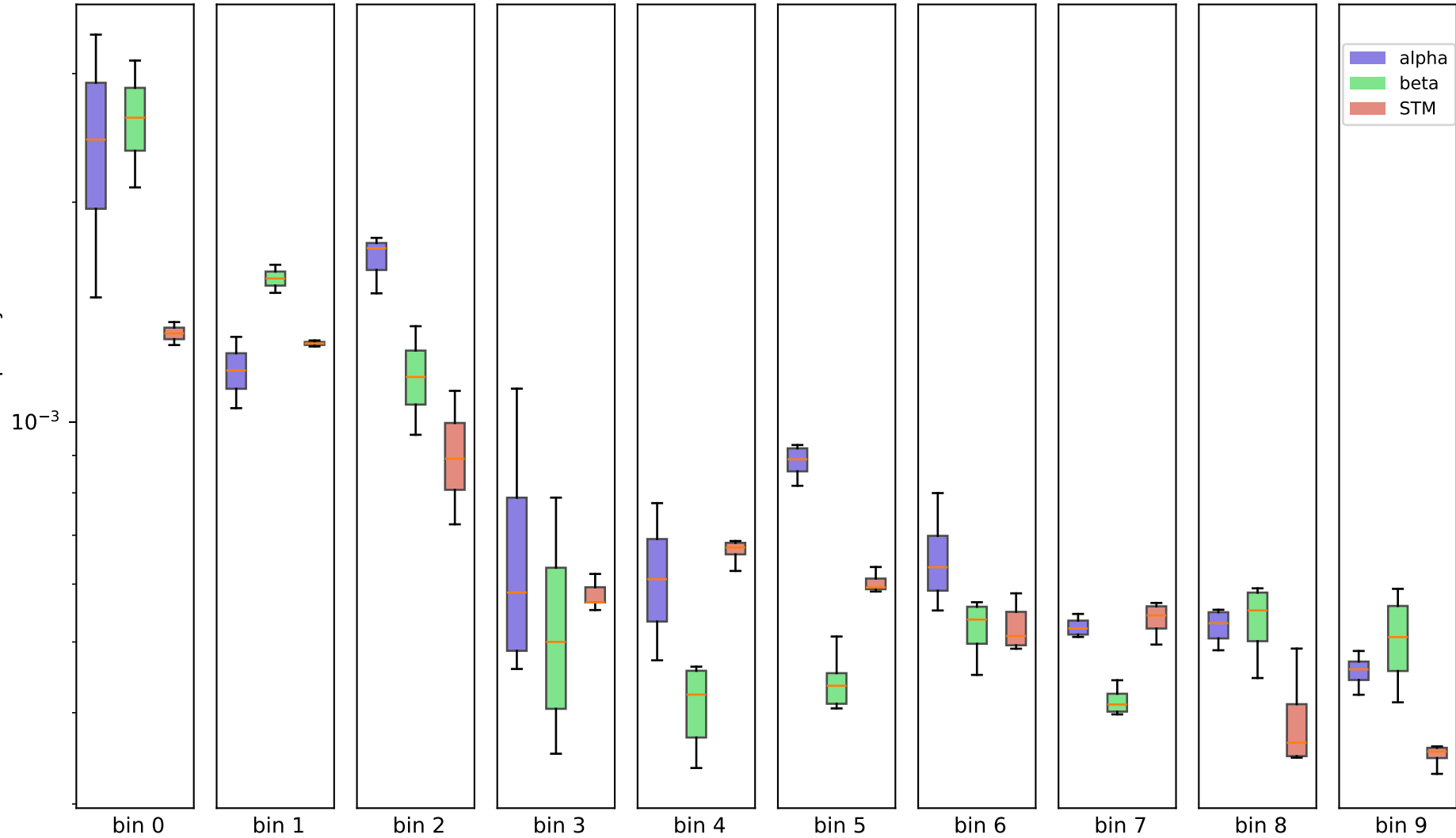
250kb - chr10, (10 bins) - 50k contacts per sample
