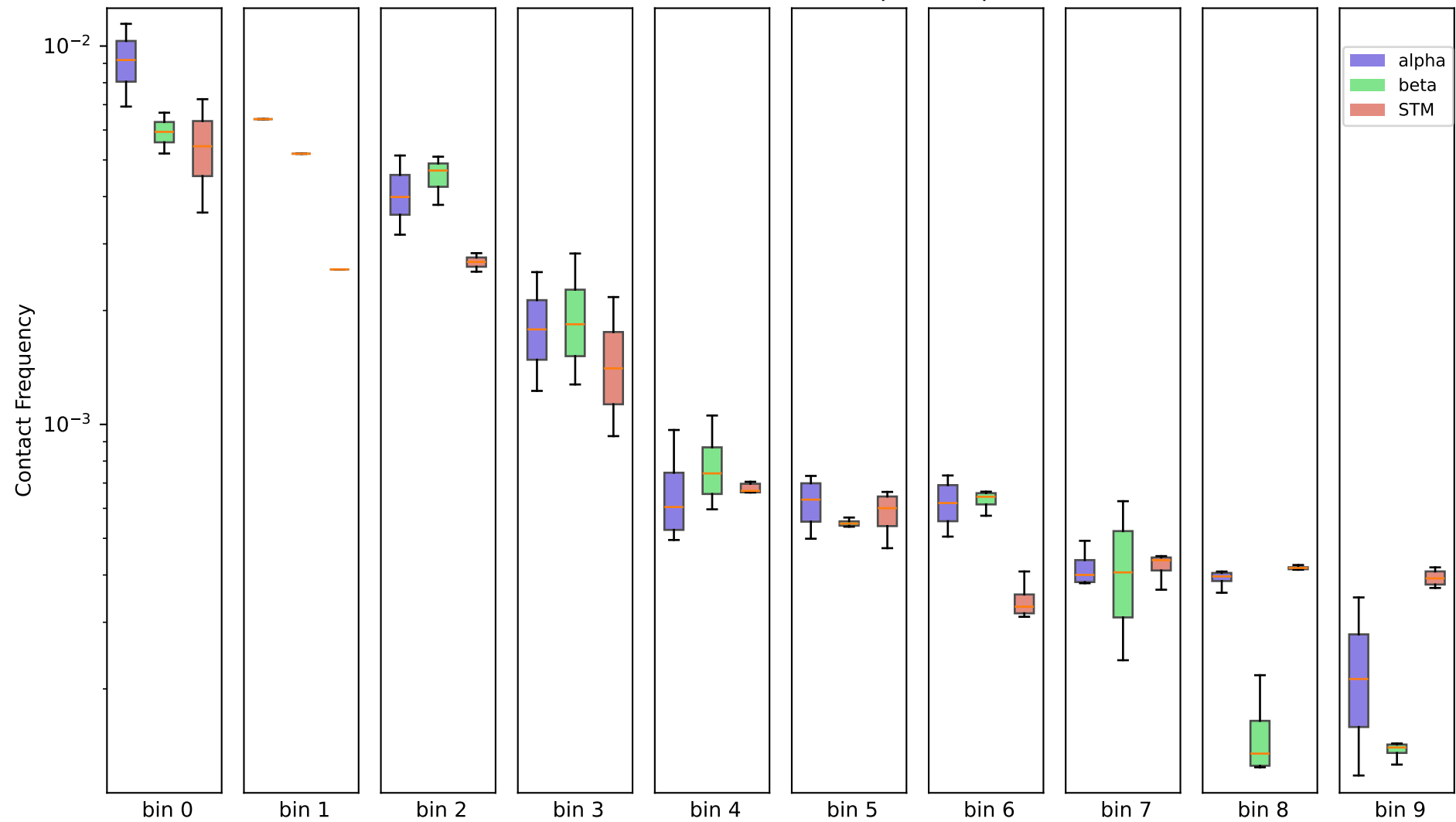
250kb - chr9, (10 bins) - 50k contacts per sample
