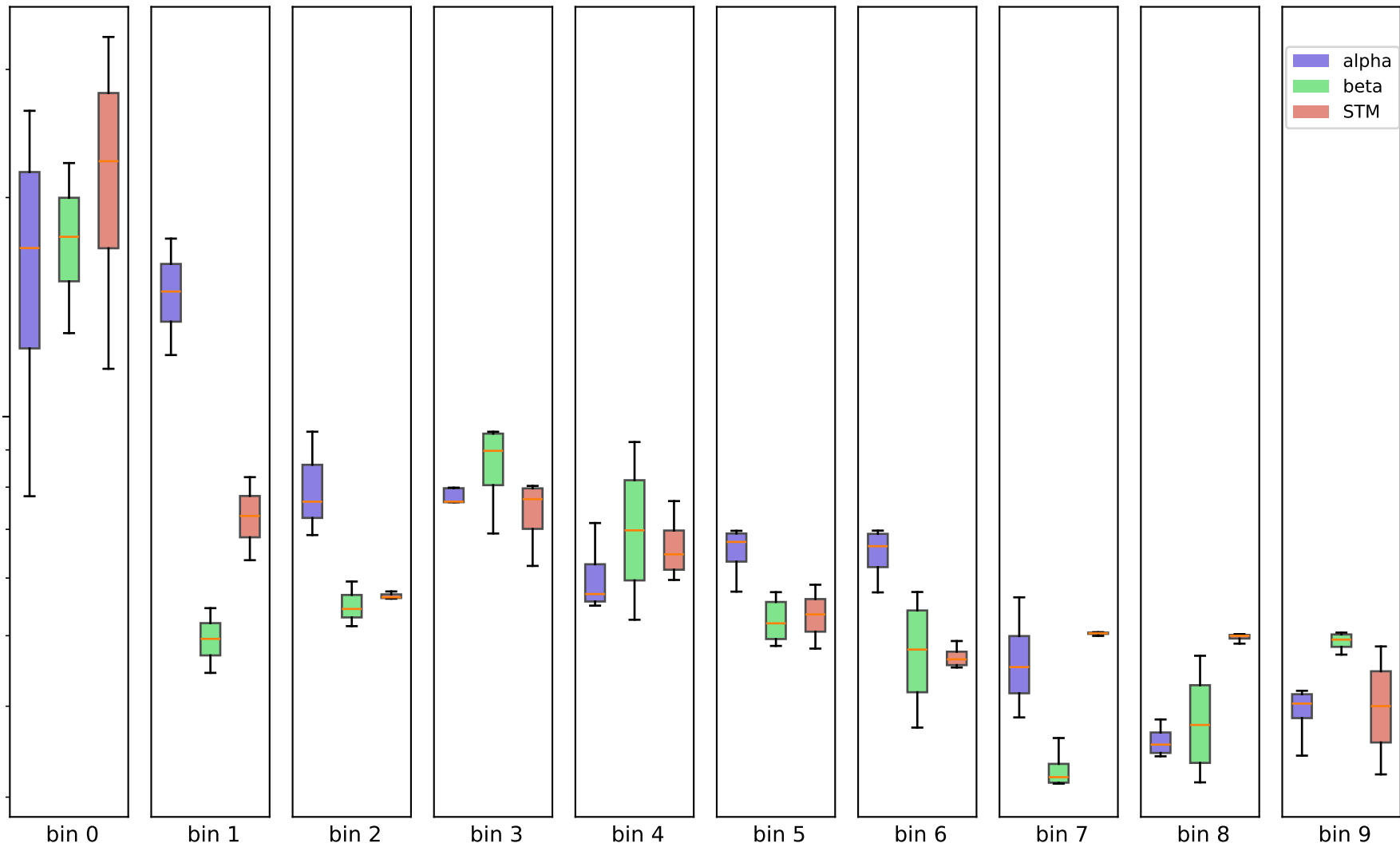
250kb - chr6, (10 bins) - 50k contacts per sample
