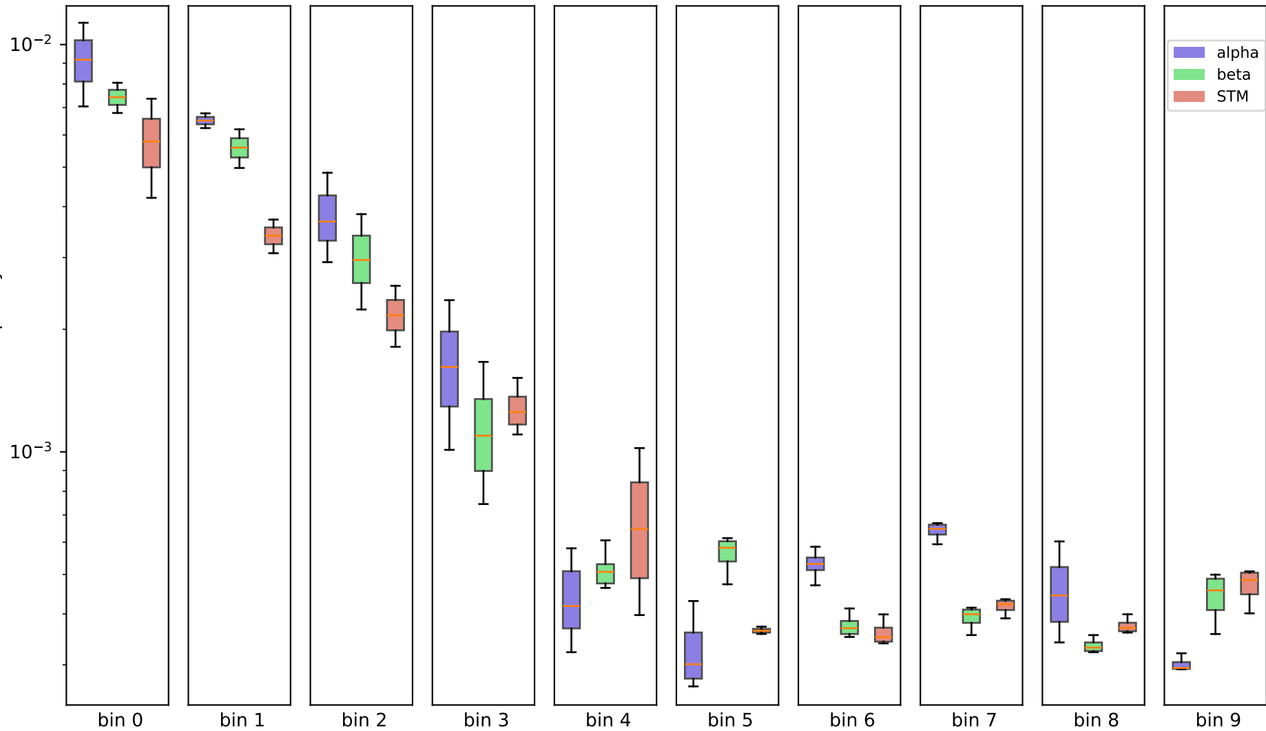
250kb - chr4, (10 bins) - 50k contacts per sample
