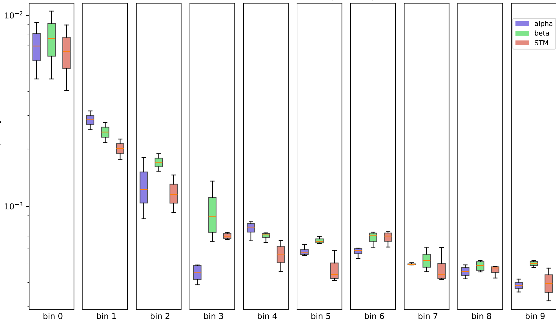
250kb - chr5, (10 bins) - 50k contacts per sample
