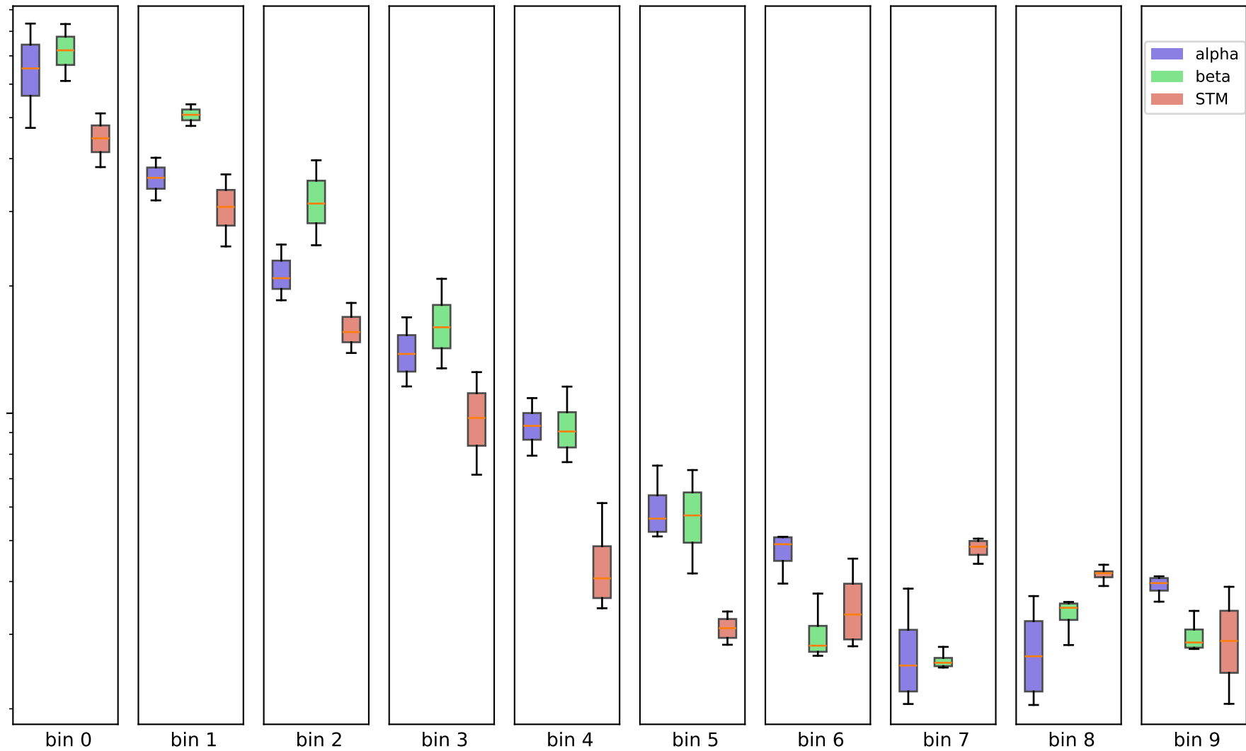
250kb - chr8, (10 bins) - 50k contacts per sample
