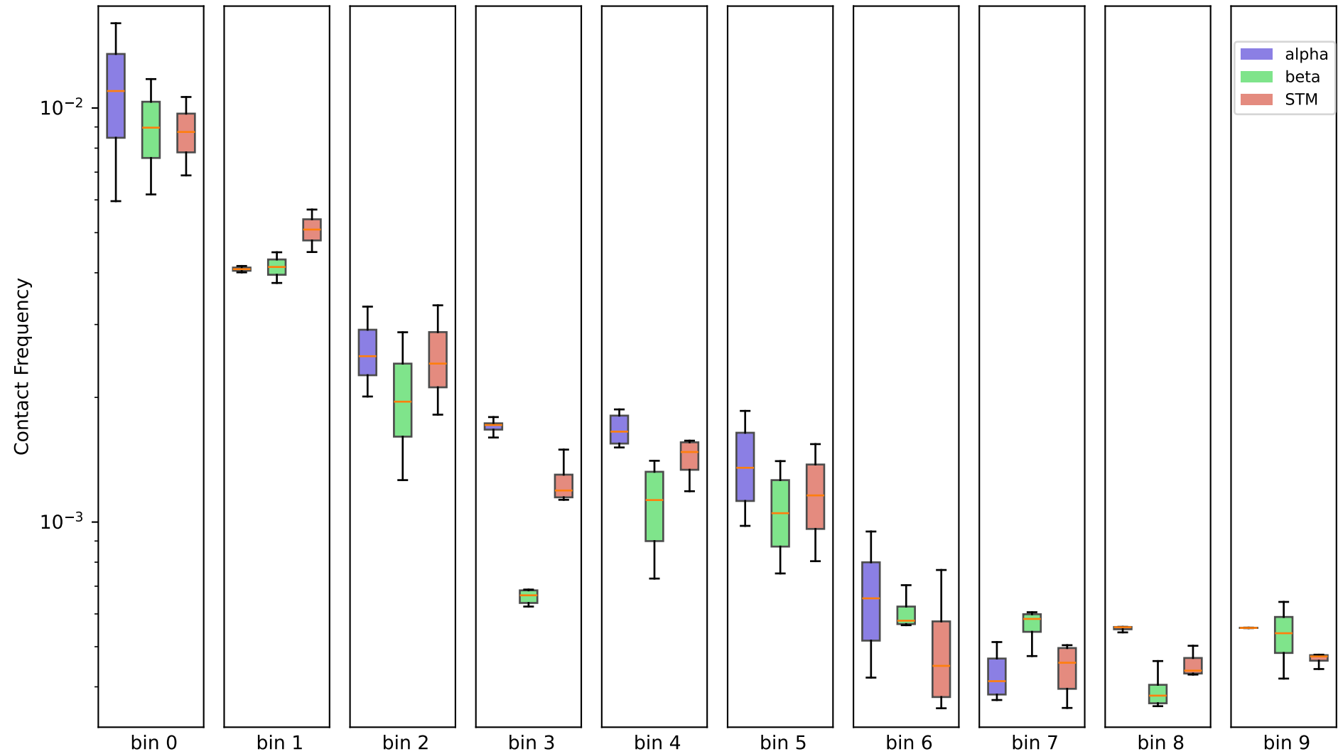
250kb - chr2, (10 bins) - 50k contacts per sample
