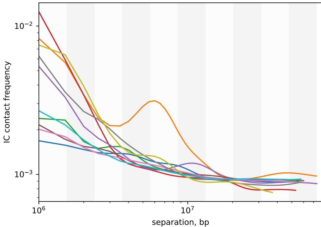
\alpha +STM 500kb , smoothed
