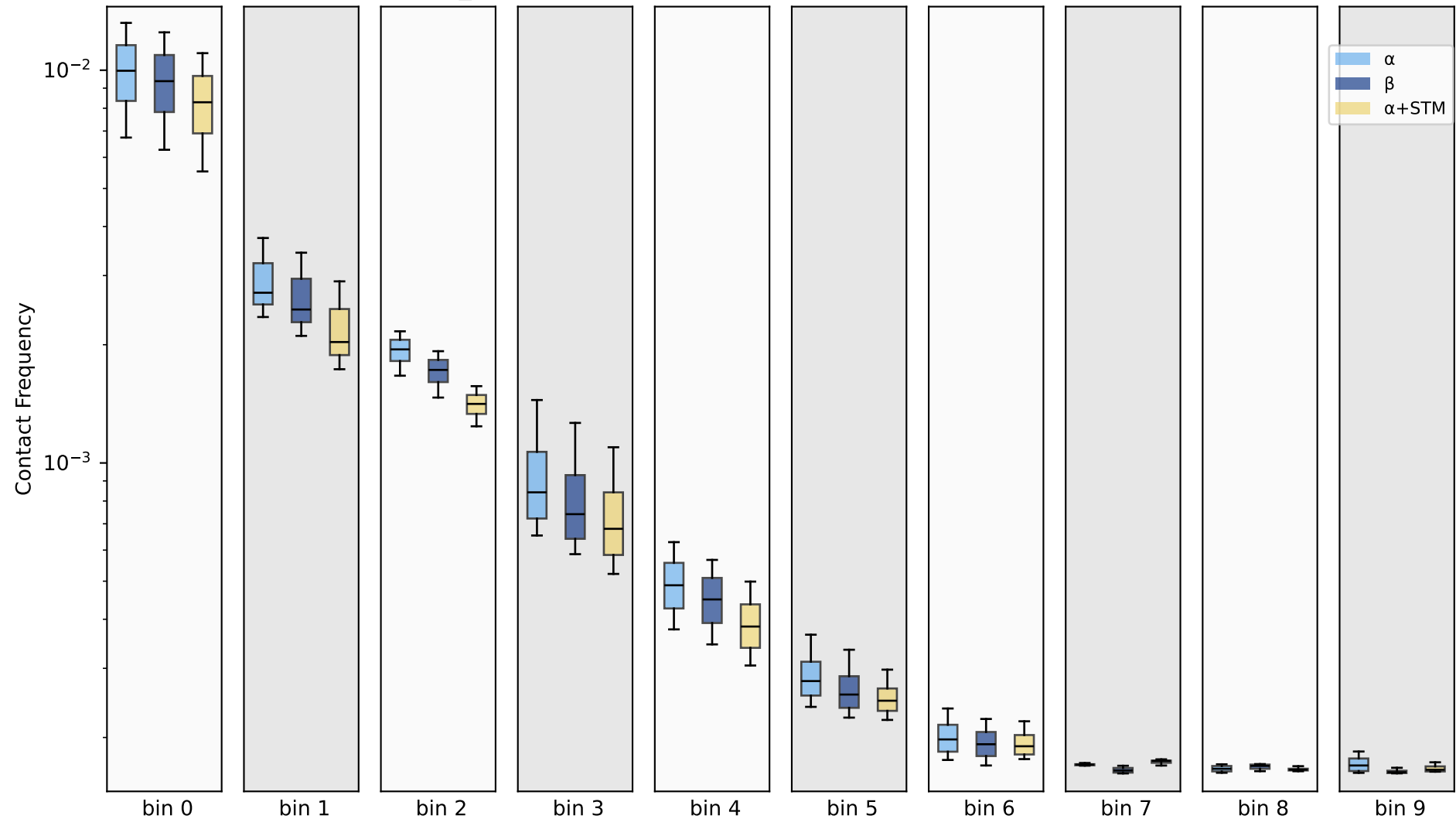
100kb - NC_047566.1, (10 bins) - 150k cis contacts per sample
