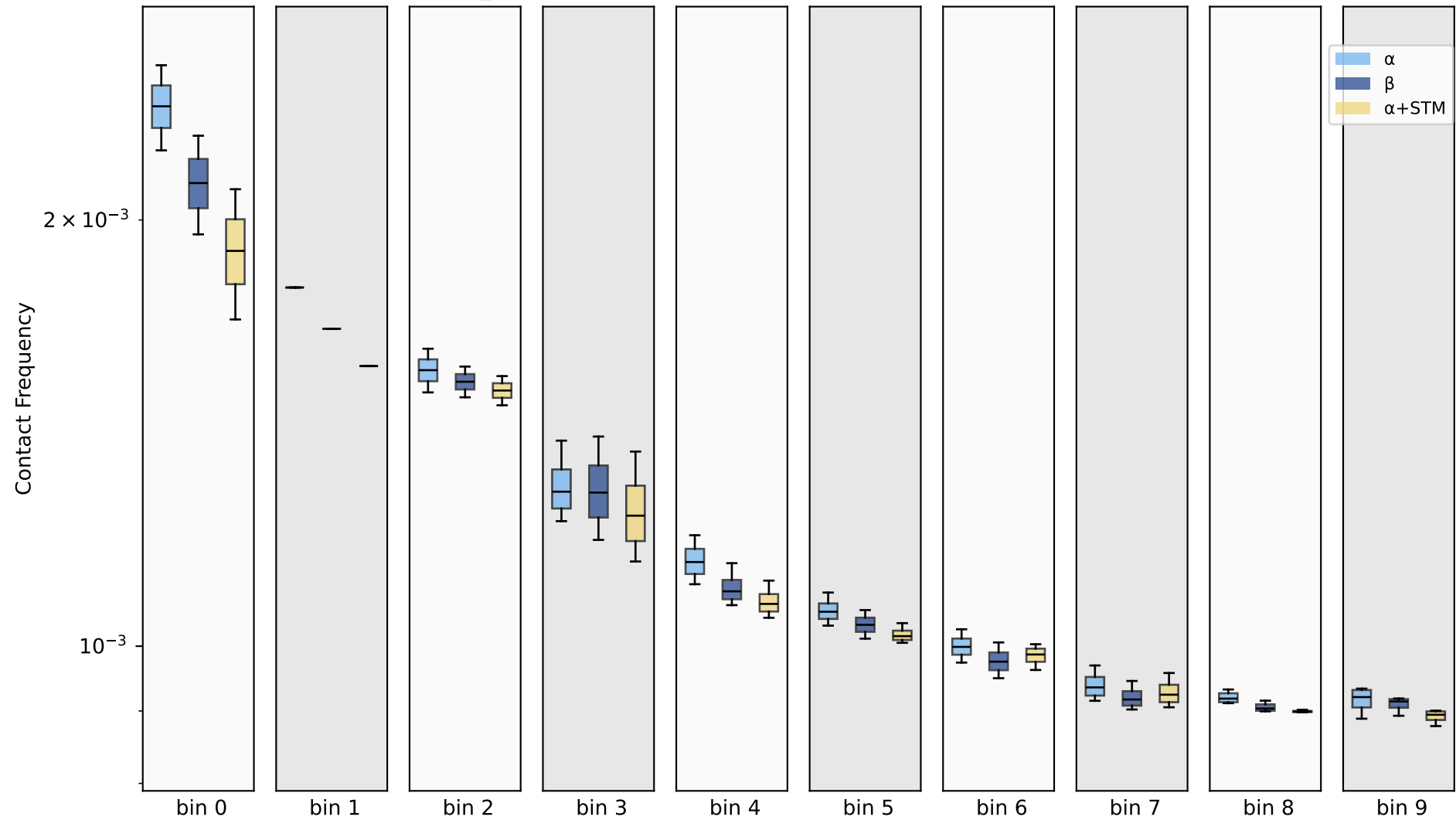
500kb - NC_047564.1, (10 bins) - 150k cis contacts per sample
