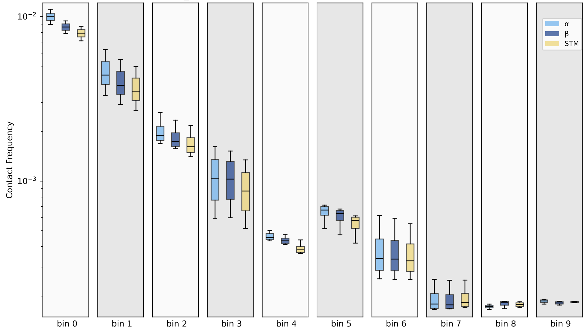
100kb - NC_047560.1, (10 bins) - 150k cis contacts per sample
