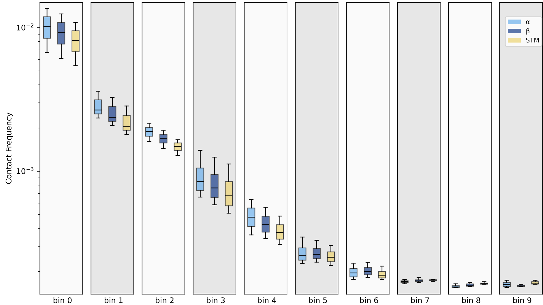
100kb - NC_047566.1, (10 bins) - 150k cis contacts per sample
