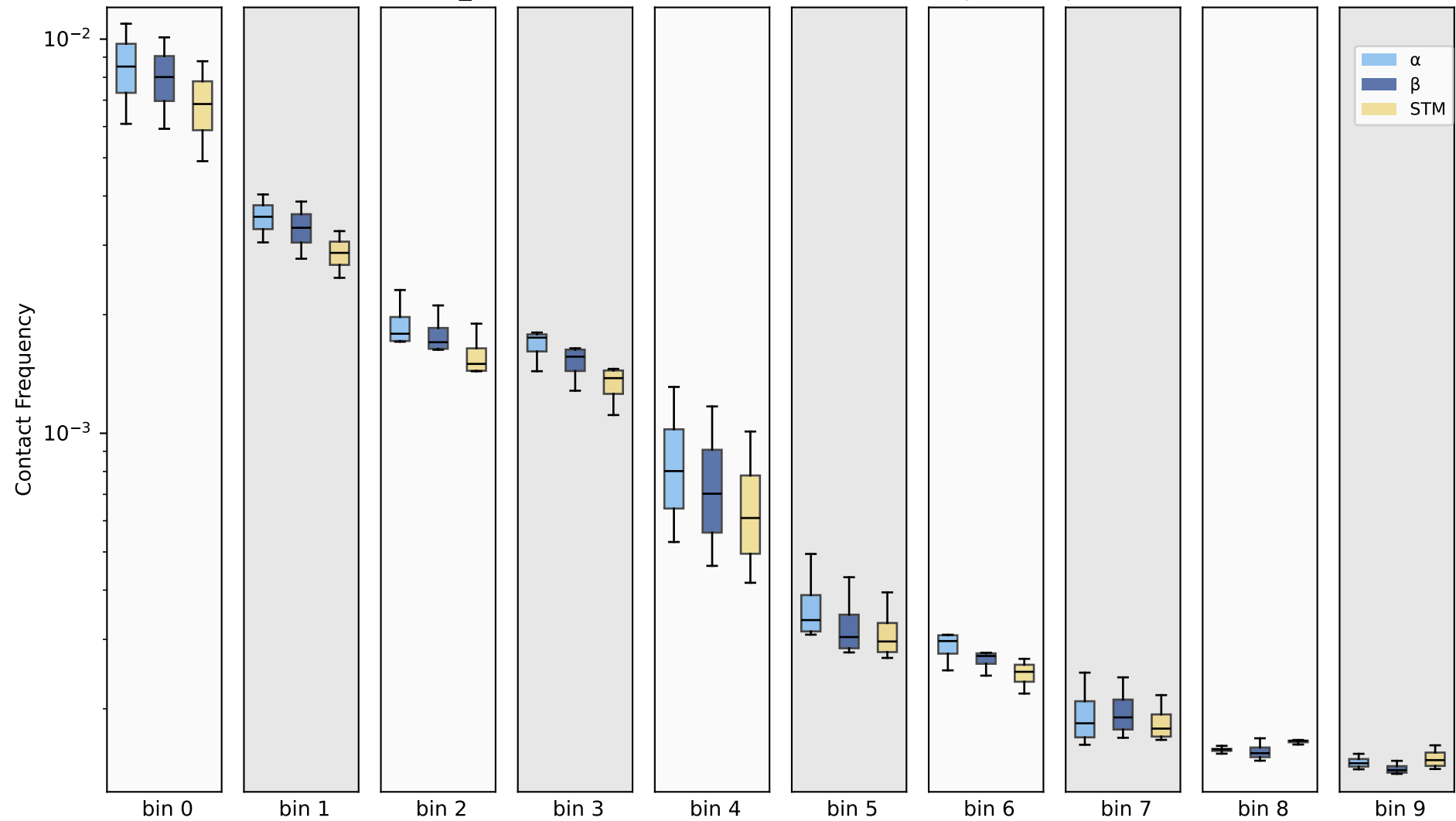
100kb - NC_047567.1, (10 bins) - 150k cis contacts per sample
