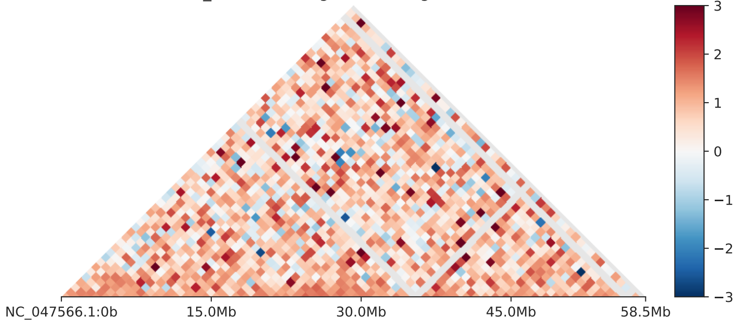
log2 fold change (insulation score)
